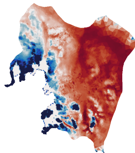
Shreve potential
