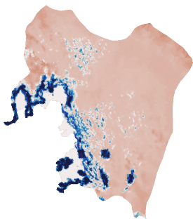
Surface slope
