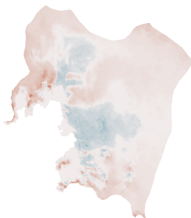
Bed slope
