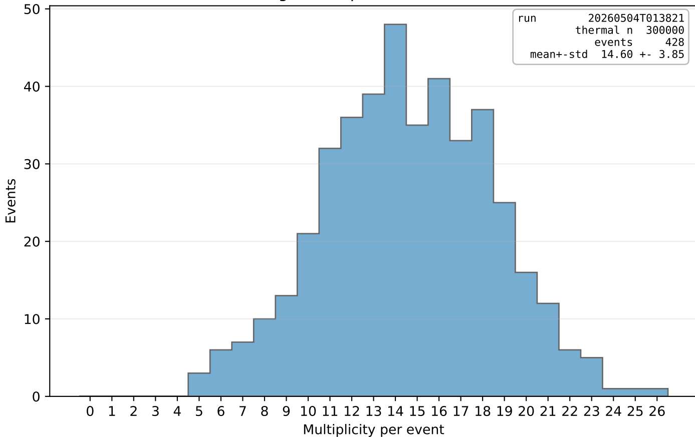
Chain ions ( \geq 2 fragments) per event - run 20260504T013821
