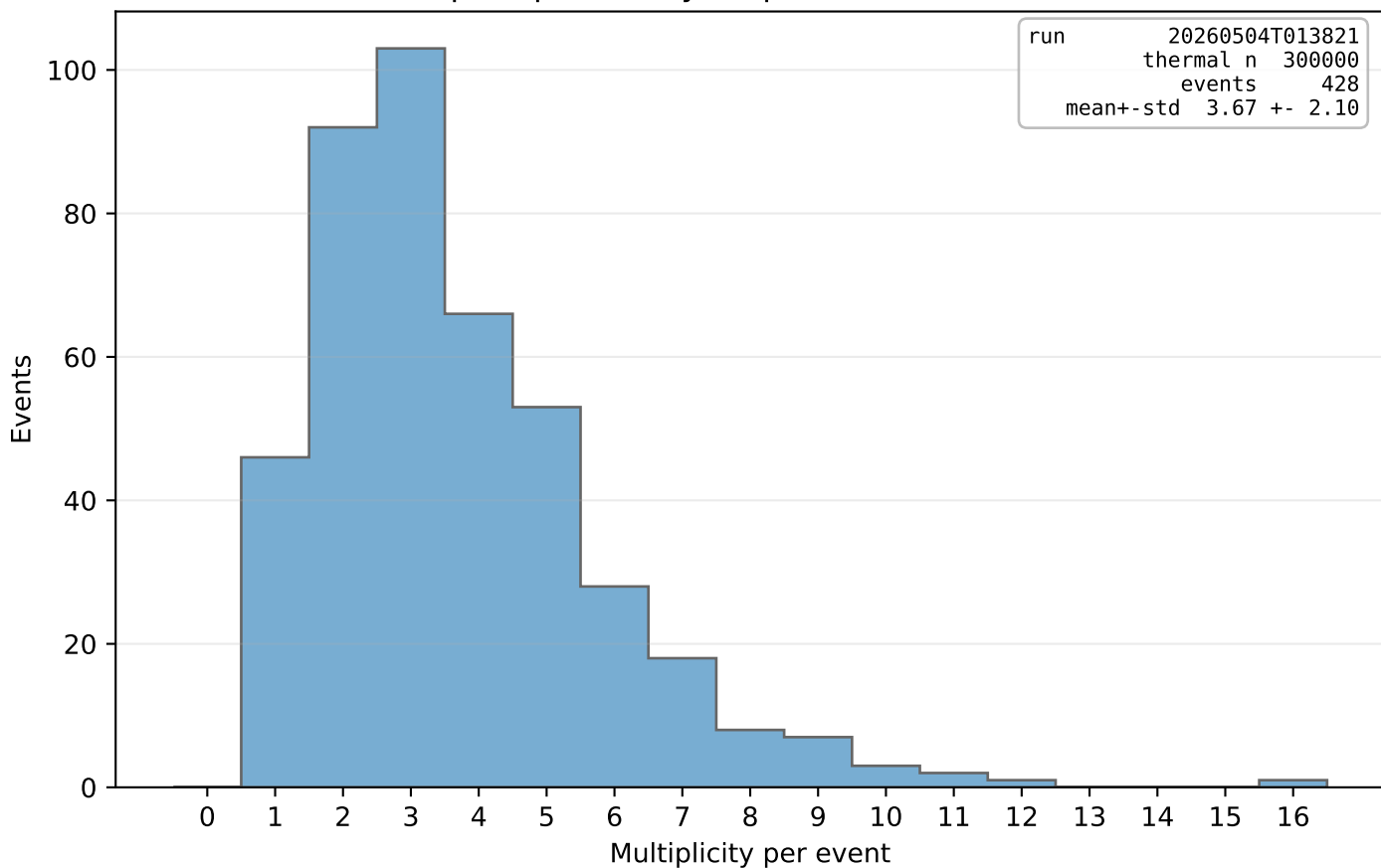
Chain neutrons (prompt + delayed) per event - run 20260504T013821
