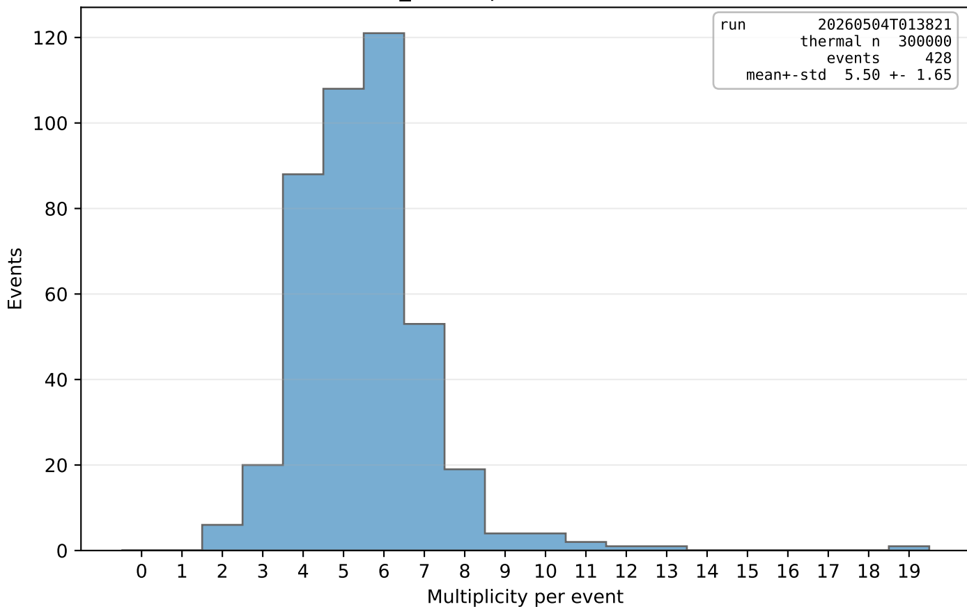
Chain other (anti-nu_e etc.) per event - run 20260504T013821
