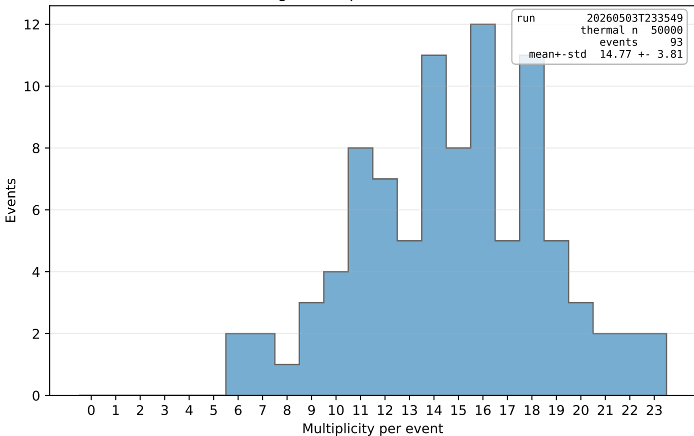
Chain ions ( \geq 2 fragments) per event - run 20260503T233549
