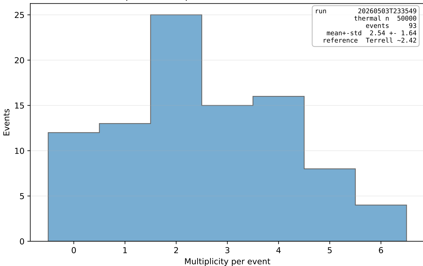
Prompt neutrons per event - run 20260503T233549
