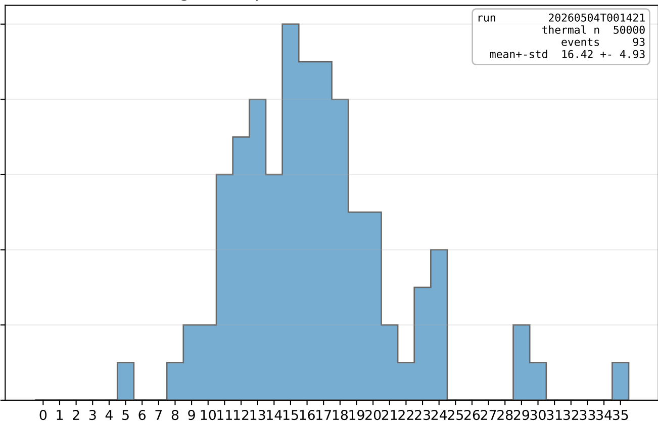
Chain gammas per event - run 20260504T001421
