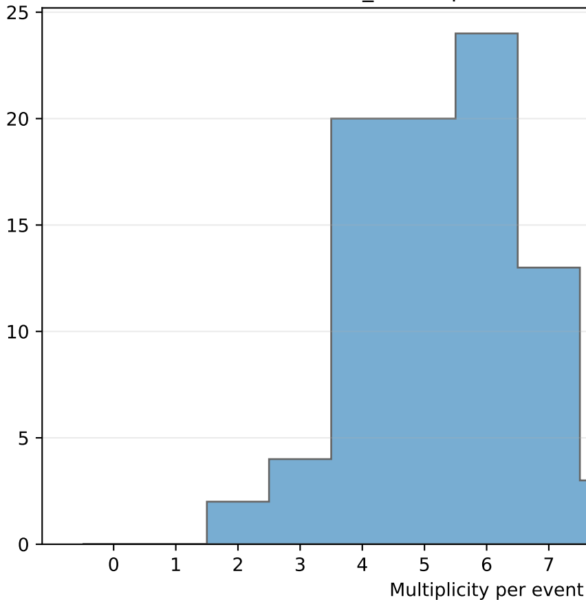
Chain other (anti-nu_e etc.) per event - run 20260504T001421
