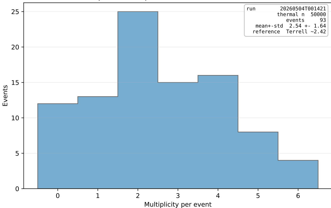
Prompt neutrons per event - run 20260504T001421
