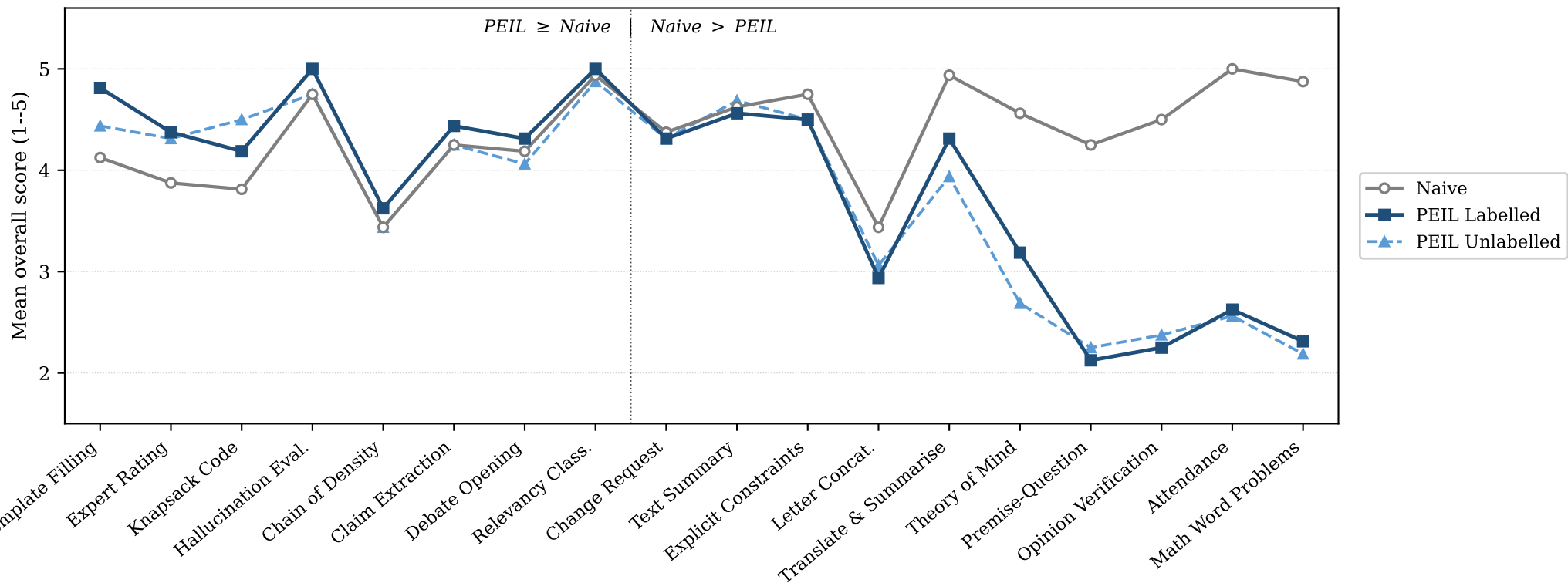
Per-pattern mean scores across four evaluated models
