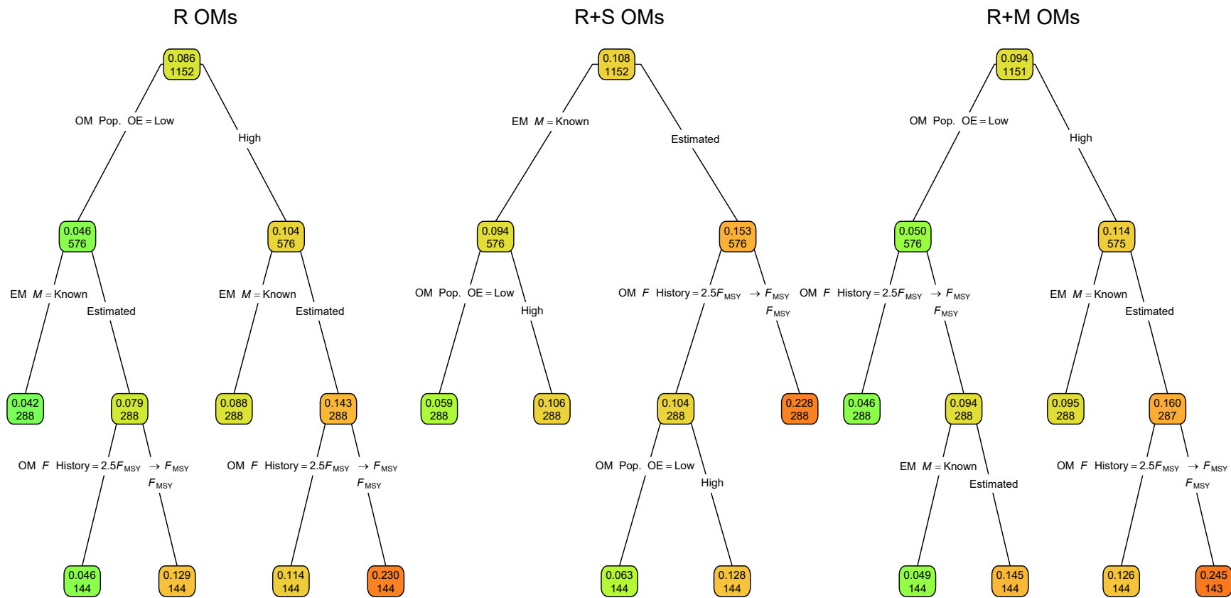
Fig. S66. Regression trees for the log-transformed RMSE of terminal year fishing mortality rate. Each node shows the median error for the corresponding subset. Lower or higher median RMSE is indicated by more green or red polygons, respectively. See Figure 1 caption and Table S1 for further details.
