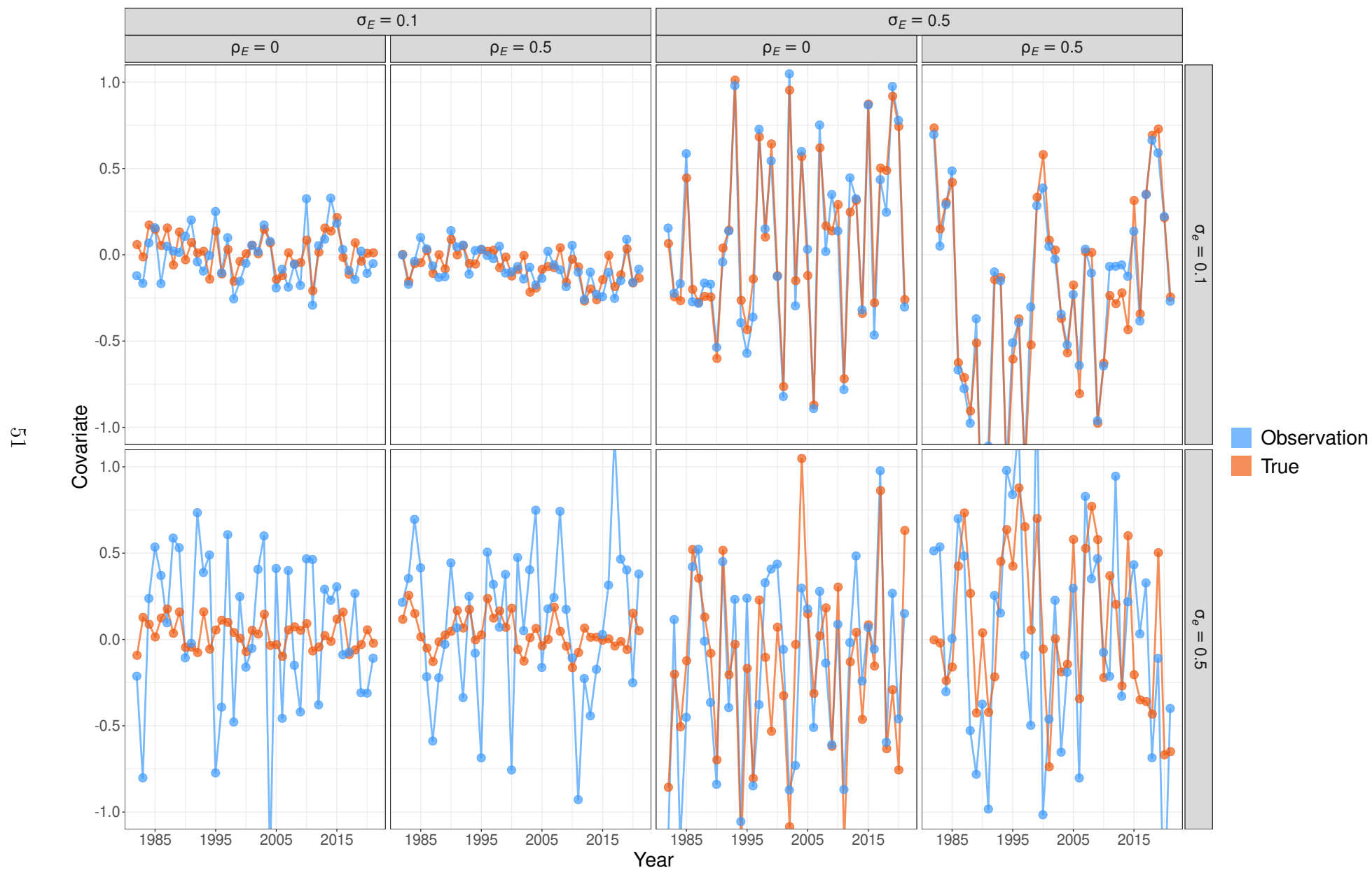
Fig. S1. Example simulations of environmental covariate latent processes and observations with different levels of observation error, and different assumptions about variability of the latent process.
