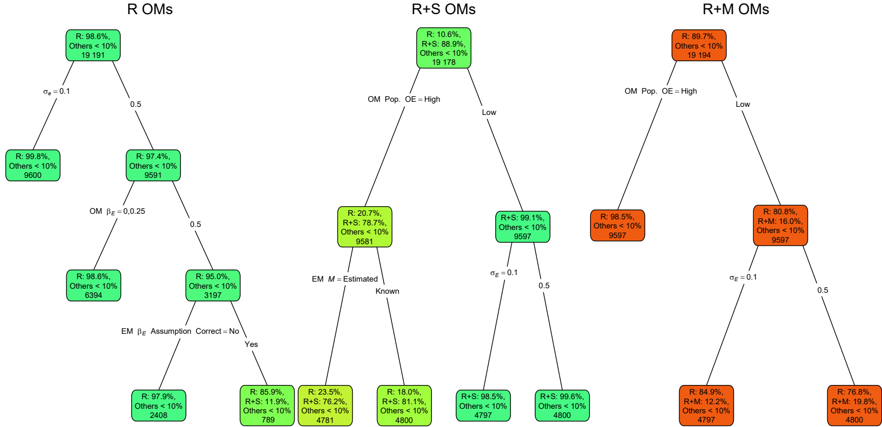
Fig. 2. Classification trees for which EM process error assumption provides the lowest AIC. Each node shows the percentage of EM fits with a given process error assumption having the lowest AIC for the corresponding subset. Lower or higher accuracy are indicated by more red or green polygons, respectively. See Figure 1 caption and Table S1 for further details.
