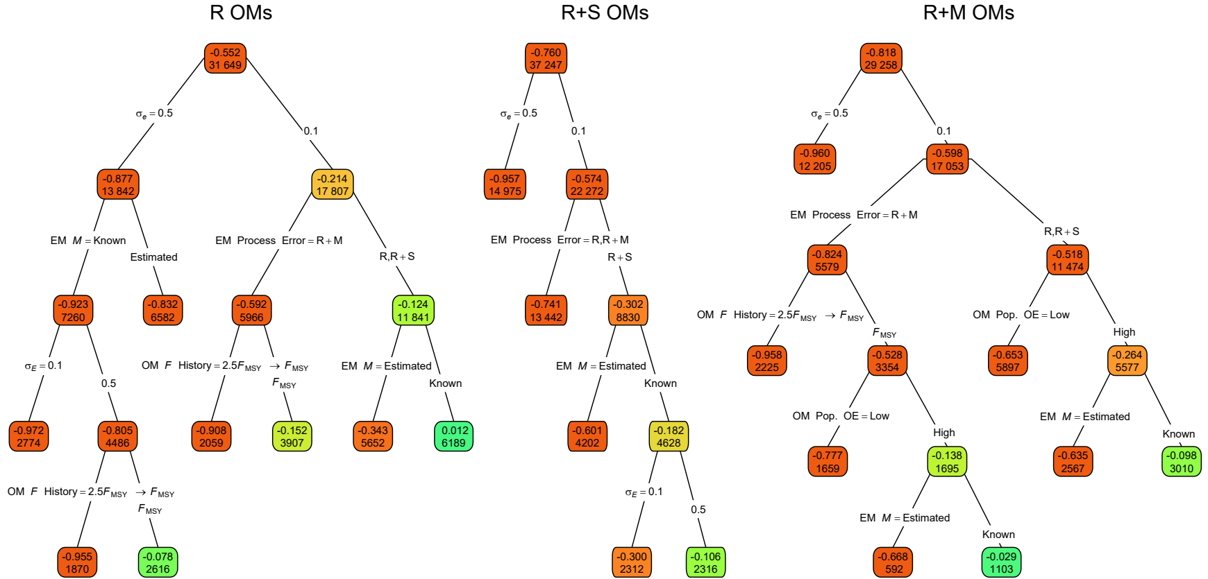
Fig. S4. Regression trees for error of the Hessian-based standard error estimates for covariate effect on M ( \widehat{SE}(\hat{\beta}_E) ). Each node shows the median error for the corresponding subset. Lower or higher absolute median errors are indicated by more green or red polygons, respectively. See Figure 1 caption and Table S1 for further details.
