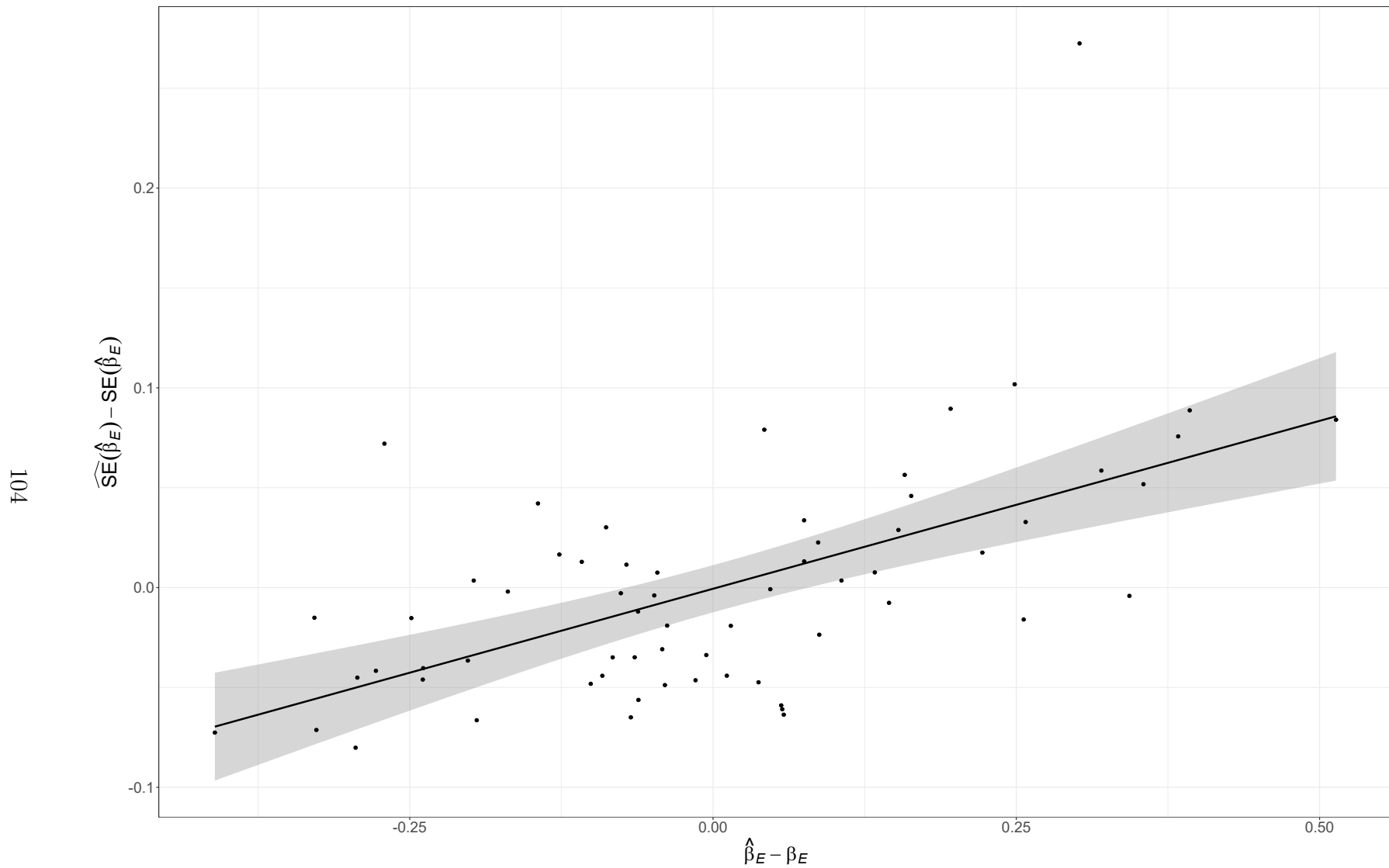
Fig. S29. Positive correlation of covariate effect estimates and Hessian-based standard error estimates for EM that also estimates the median M parameter ( \beta_M ) and has correct R+M process error assumption fitted to simulated data from the OM with R+M process errors, temporal contrast in fishing pressure, low observation uncertainty for both population ( LowOE ) and covariate observations ( \sigma_e = 0.1 ), high and uncorrelated temporal variability in the true covariate ( \sigma_E = 0.5 and \rho_E = 0 ), and the strongest covariate effect on M ( \beta_E = 0.5 ).
