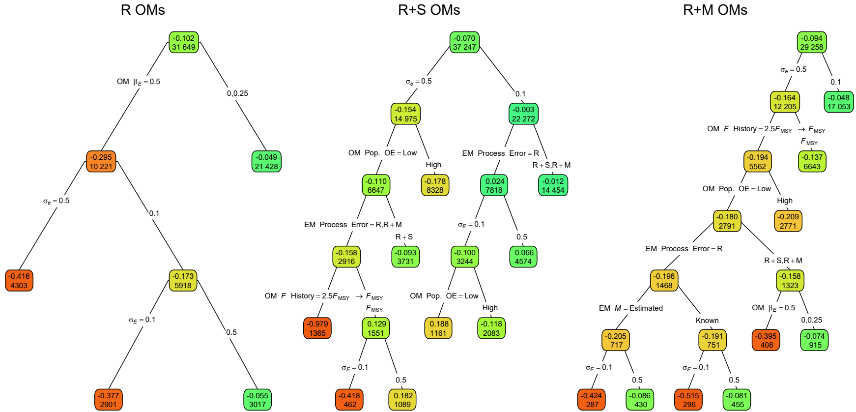
Fig. 4. Regression trees for estimation error of the covariate effect on M ( \hat{\beta}_E ). Each node shows the median error (top) for the corresponding subset. Lower or higher absolute median error are indicated by more green or red polygons, respectively. See Figure 1 caption and Table S1 for further details.
