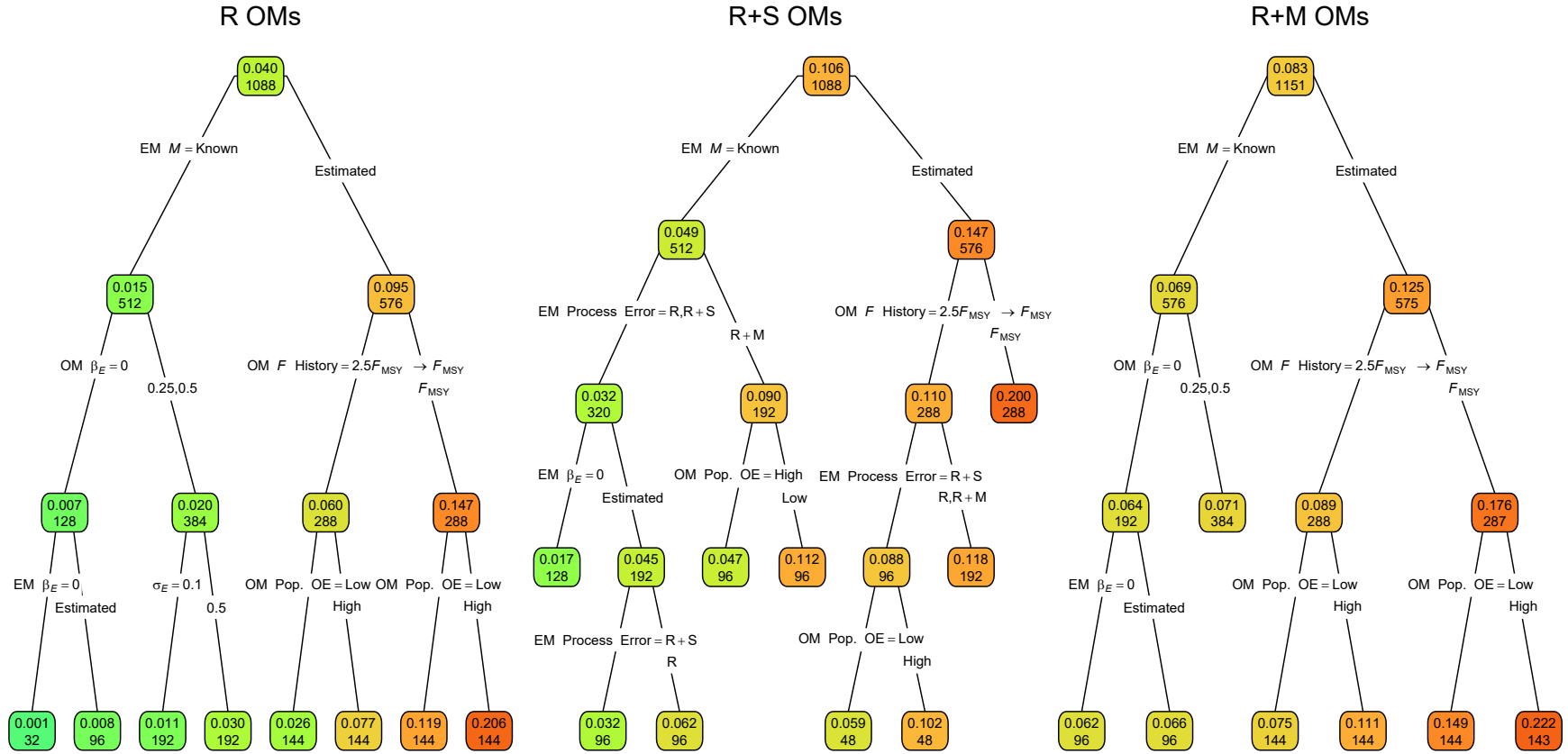
Fig. S6. Regression trees for the log-transformed RMSE of terminal year M . Each node shows the median error (top) and number of observations (bottom) for the corresponding subset. Lower or higher median RMSE are indicated by more green or red polygons, respectively. See Figure 1 caption and Table S1 for further details.
