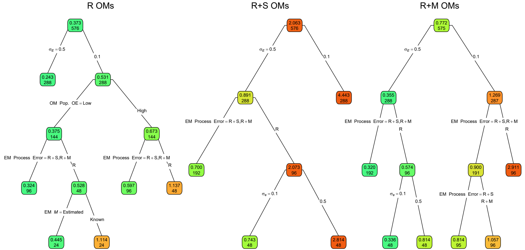
Fig. S25. Regression trees for the log-transformed RMSE of covariate effect on M ( \text{RMSE}(\hat{\beta}_E) ). Each node shows the median error for the corresponding subset. Lower or higher median RMSE are indicated by more green or red polygons, respectively. See Figure 1 caption and Table S1 for further details.
