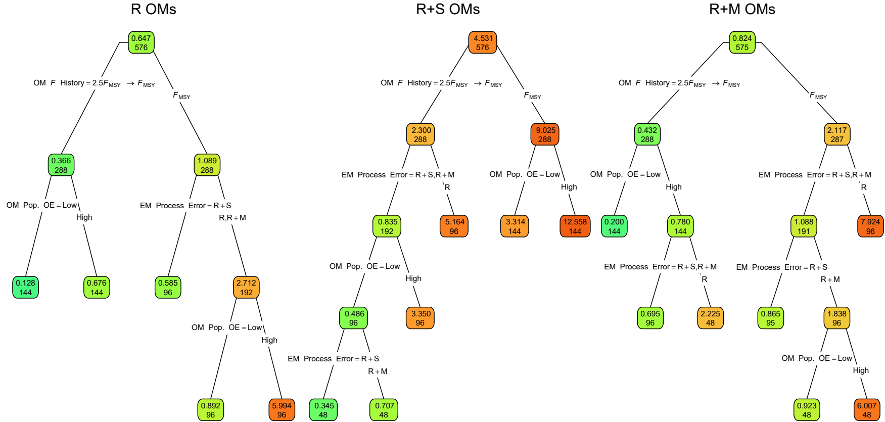
Fig. S40. Regression trees for the log-transformed RMSE of estimates for the median M parameter ( \text{RMSE}(\hat{\beta}_M) ). Each node shows the median error for the corresponding subset. Lower or higher median RMSE are indicated by more green or red polygons, respectively. See Figure 1 caption and Table S1 for further details.
