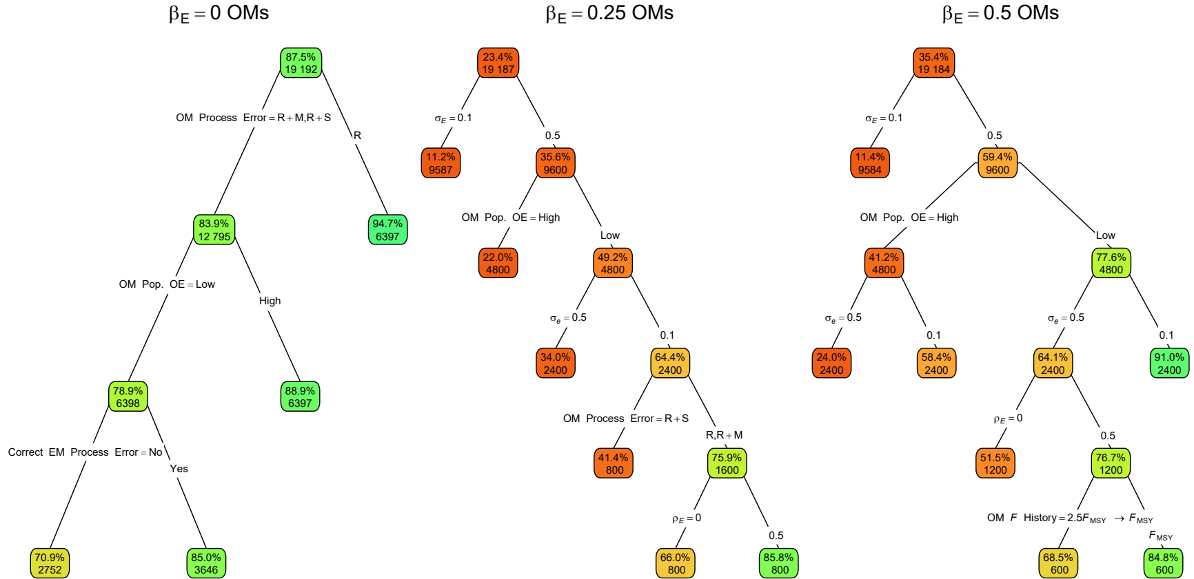
Fig. 3. Classification trees for whether the correct EM assumption for covariate effect on M (no effect with OM \beta_E = 0 or estimated effect when OM \beta_E > 0 ) provides the lowest AIC for OMs assuming values for \beta_E of 0, 0.25, and 0.5. Nodes denote the percentage of EMs with the correct assumption and lowest AIC for the corresponding subset. Lower or higher accuracy are indicated by more red or green polygons, respectively. See Figure 1 caption and Table S1 for further details.
