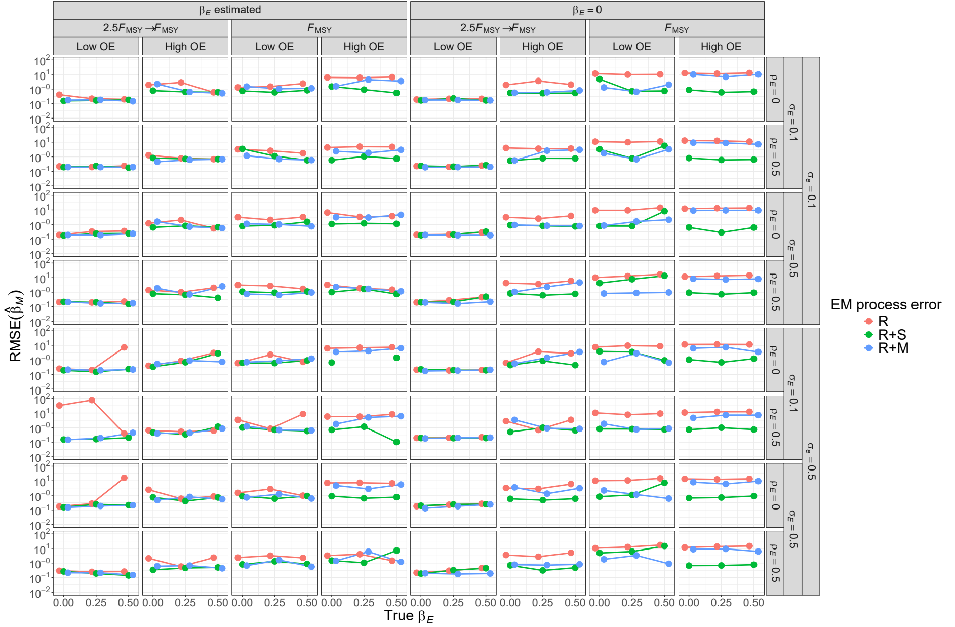
Fig. S43. For R+M OM, RMSE of estimates of \beta_M from fitting EMs with alternative process error assumptions and treatment of covariate effect ( \beta_E = 0 or estimated).
