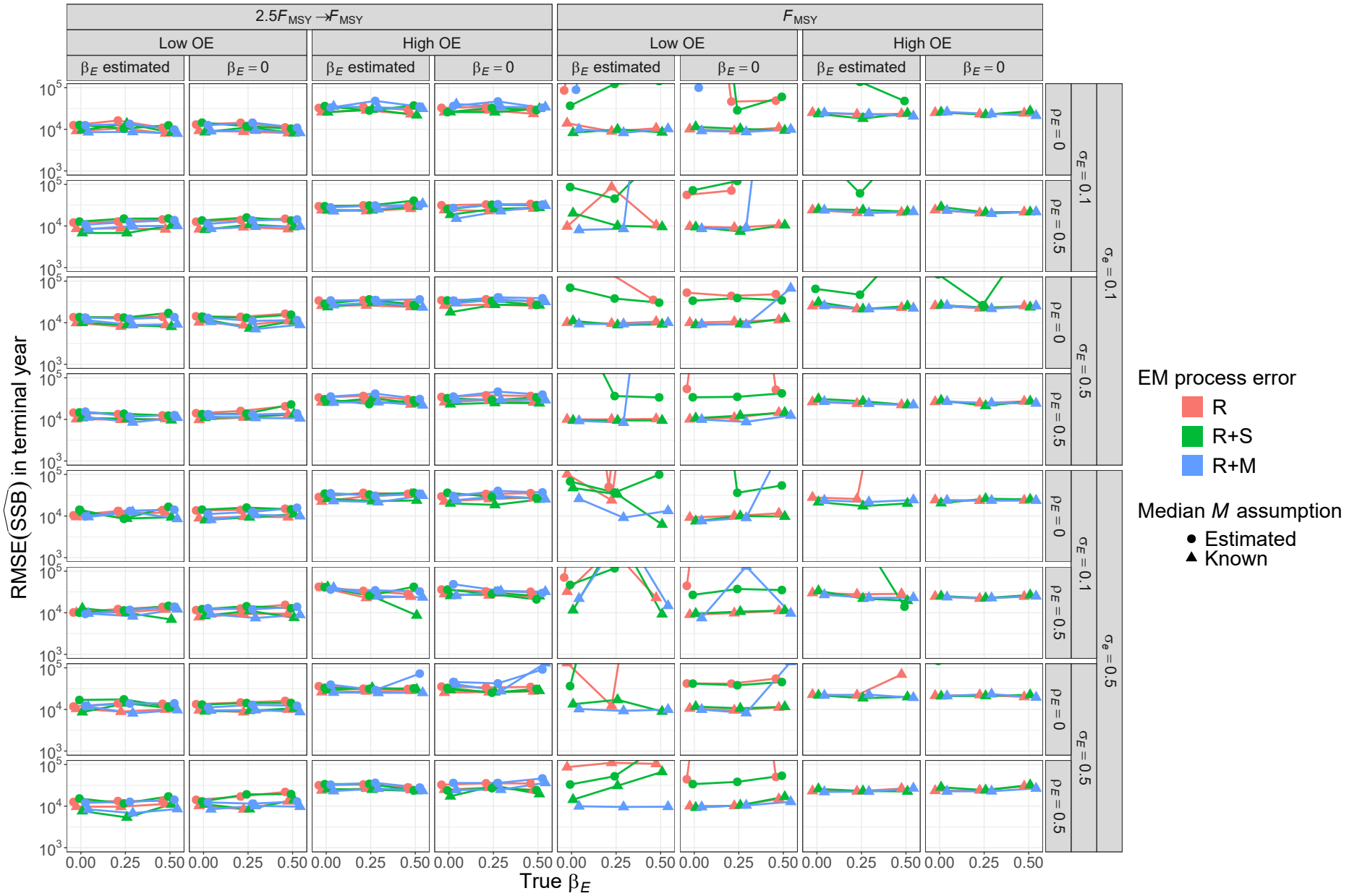
Fig. S58. For R+M OMs, RMSE of estimates of SSB in the terminal year for EMs with alternative process error assumptions, treatment of covariate effect ( \beta_E = 0 or estimated), and treatment of median M parameter ( \beta_M estimated or known).
