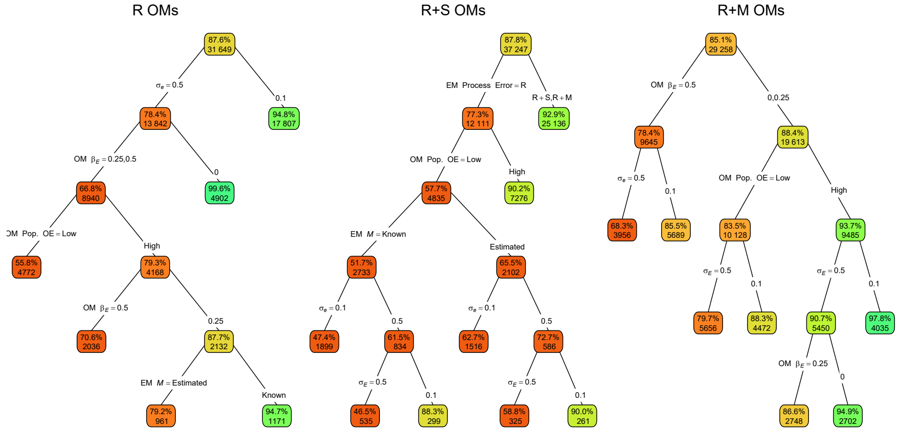
Fig. 5. Classification trees for whether confidence intervals (CIs) for the estimated covariate effects on M ( \beta_E ) included the true value. Each node shows the percentage of CIs that include the true value for the corresponding subset. Higher or lower percentages are indicated by more green or red polygons, respectively. See Figure 1 caption and Table S1 for further details.
