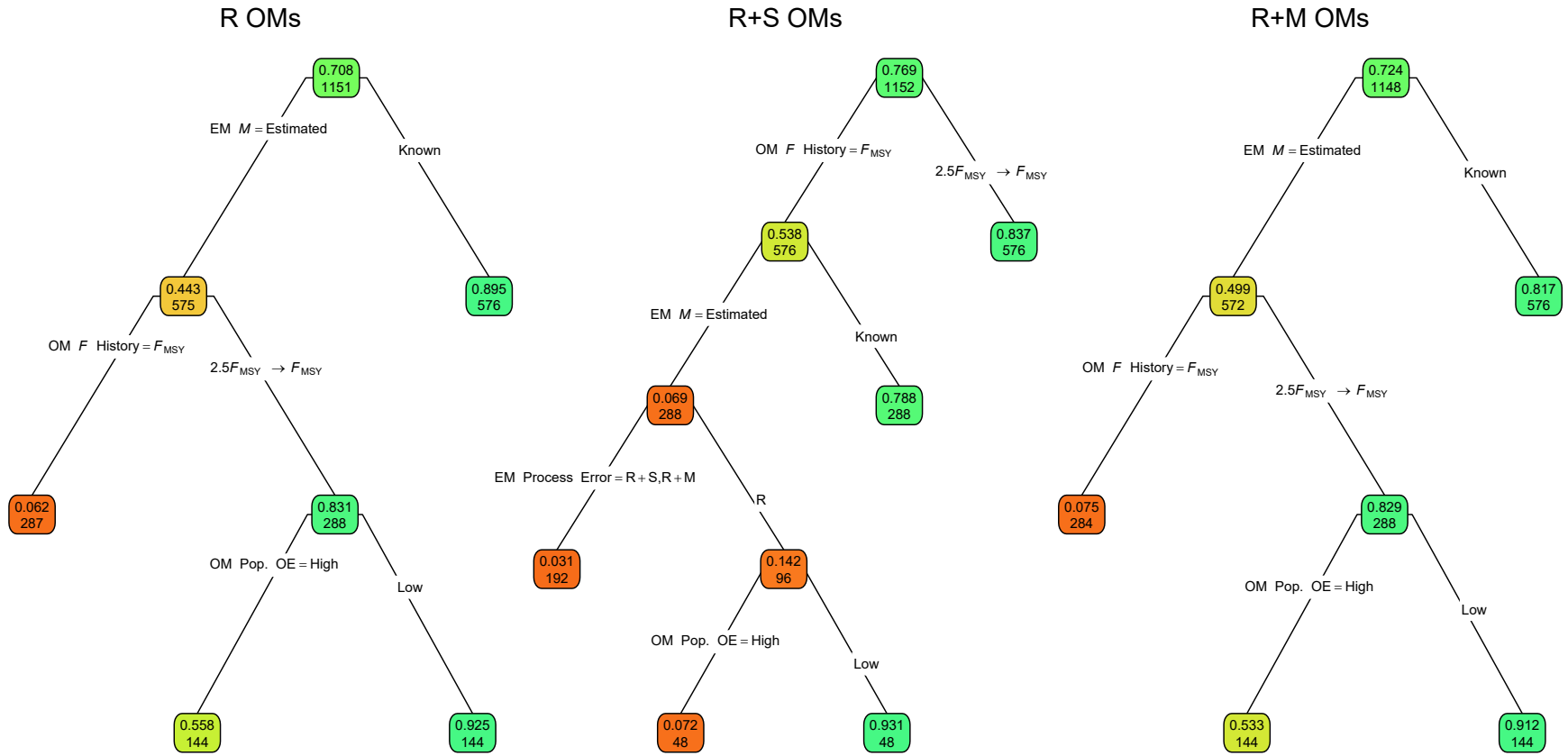
Fig. S9. Regression trees for the correlation of terminal year SSB estimates and true values. Each node shows the median error for the corresponding subset. Lower or higher median correlations are indicated by more red or green polygons, respectively. See Figure 1 caption and Table S1 for further details.
