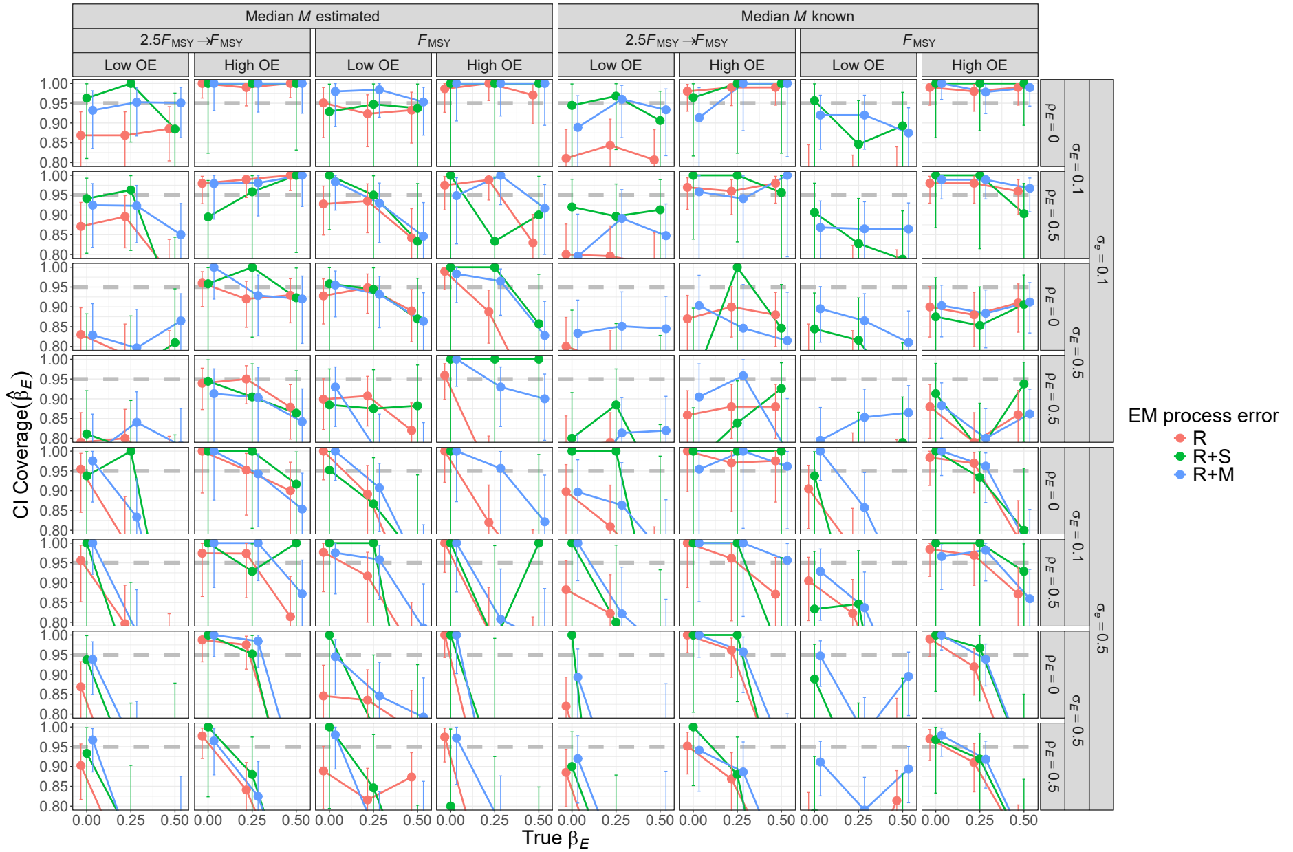
Fig. S24. For R+M OMs, probability of 95% confidence interval for \beta_E containing the true value for EMs with alternative process error assumptions and treatment of median natural mortality \mathcal{M} ( e_M^\beta known or estimated). Vertical lines represent 95% confidence intervals.
