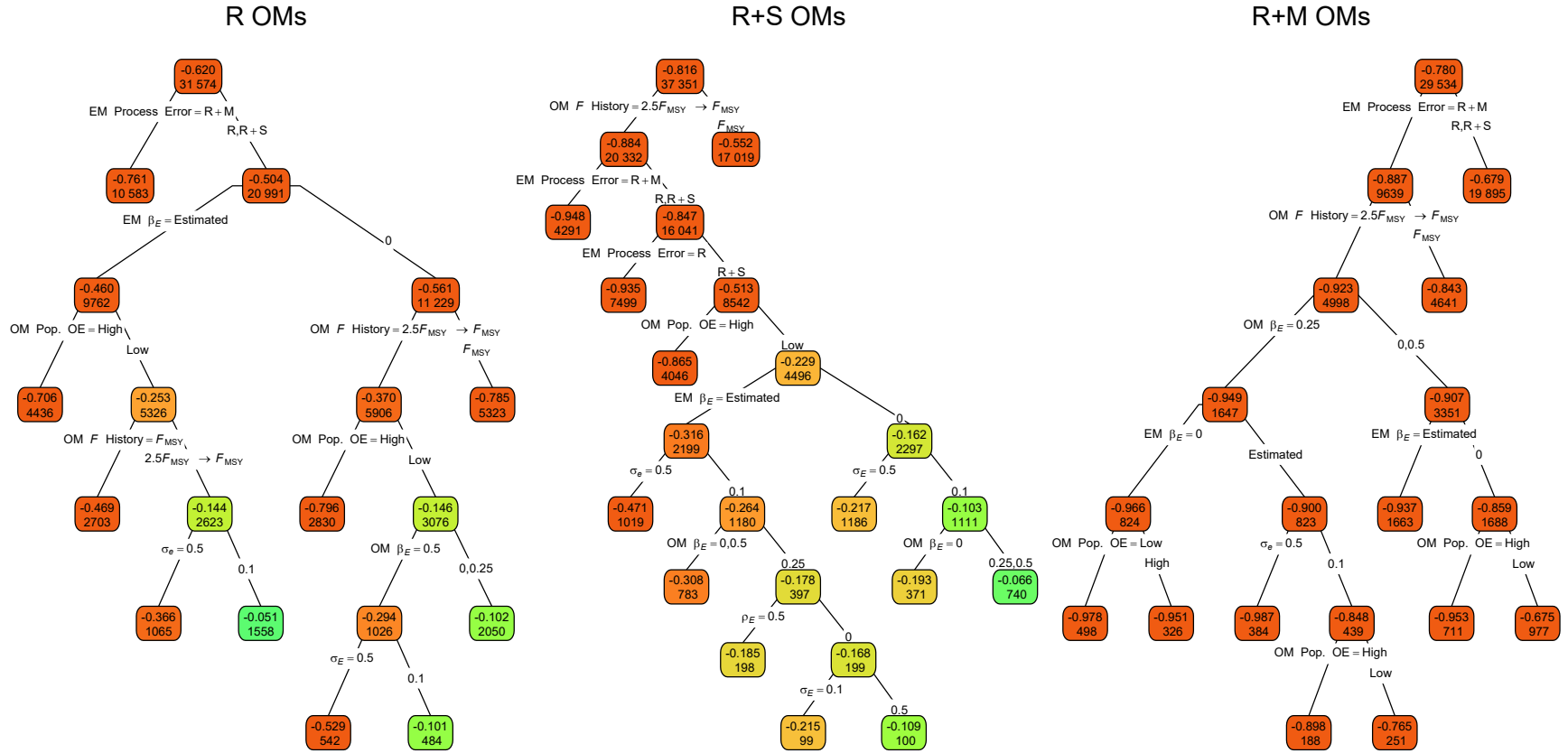
Fig. S7. Regression trees for errors of the Hessian-based standard error estimates for median M parameter ( \widehat{SE}(\hat{\beta}_M) ). Each node shows the median error for the corresponding subset. Lower or higher absolute median absolute errors of the process error assumption are indicated by more green or red polygons, respectively. See Figure 1 caption and Table S1 for further details.
