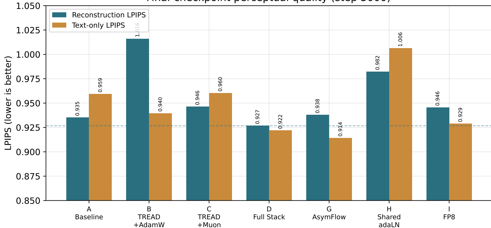
Final-checkpoint perceptual quality (step 5000)
