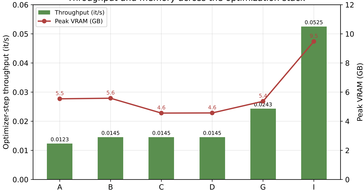
Throughput and memory across the optimization stack
