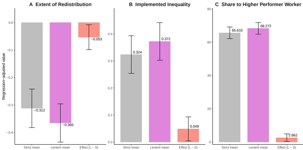
Figure 2: Inflated feedback reduces support for redistribution. Bars show regression-adjusted means ( \pm 95\% confidence intervals) from OLS models including controls for task score, baseline confidence, and education level. The first two bars display adjusted means under strict and lenient evaluations, and the third bar shows the treatment effect (Lenient – Strict). The Extent of Redistribution (Panel A) is a measure between -1 and 1 , where -1 allocates all to the higher performer (Worker One) and +1 allocates all to the lower performer (Worker Two). Implemented Inequality (Panel B) is the absolute counterpart measure and ranges from 0 to 1 . Panel C, the Share Allocated to the Higher Performer, is the share given to the higher performer worker, plotted in percentage points.
