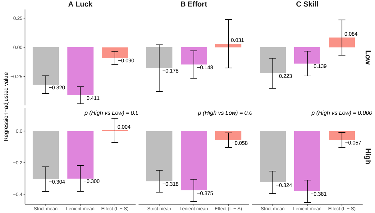
Figure 4: Heterogeneity by perceived importance of luck, effort, and skill. Bars show regression-adjusted means ( \pm 95\% confidence intervals) from OLS models including controls for task score, baseline confidence, and education level. The first two bars display adjusted means under strict and lenient evaluations, and the third bar shows the treatment effect (Lenient – Strict) on the Extent of Redistribution. Panels are split by whether participants judged luck, effort, or skill to matter “not at all” or “a little” ( Low importance ) versus “somewhat,” “quite a bit,” or “very much” ( High importance ) for performance on the task. p(High vs Low) in High-importance panels reports the Welch t-test p-value comparing the treatment effect between High and Low groups (treated subsample).
