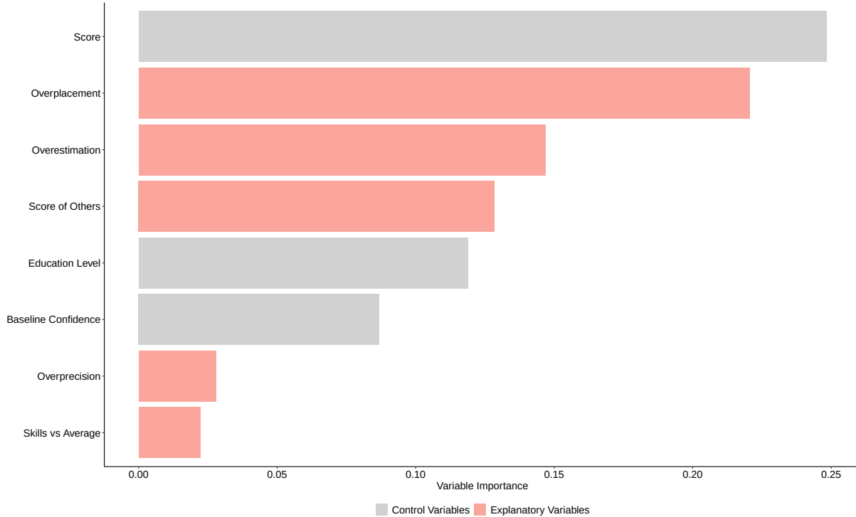
Extended Data Figure 1 — Overplacement is more predictive than overestimation in conditional average treatment effects. Bars show variable importance scores from a causal forest predicting the conditional average treatment effect of inflated feedback on the Extent of Redistribution. Variables are grouped into Explanatory variables (salmon) and Control variables (grey). Among the Explanatory variables, Overplacement contributes most strongly to explaining heterogeneity in treatment effects, compared to overestimation and other belief measures.
