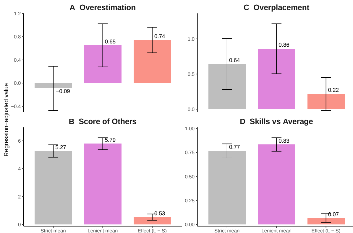
Figure 1: Inflated feedback increases confidence measures. Bars show regression-adjusted means ( \pm 95\% confidence intervals) from OLS models including controls for task score, baseline confidence, and education level. The first two bars display adjusted means under strict and lenient evaluations, and the third bar shows the treatment effect (Lenient – Strict). Overestimation (Panel A) measures the gap between actual and perceived scores. Score of Others (Panel B) reflects the perceived scores of participants. Panel C captures the difference between perceived and actual score differences relative to the modal score. Panel D is a binary variable indicating whether individuals perceive their skills as weakly better than the average US skill level.
