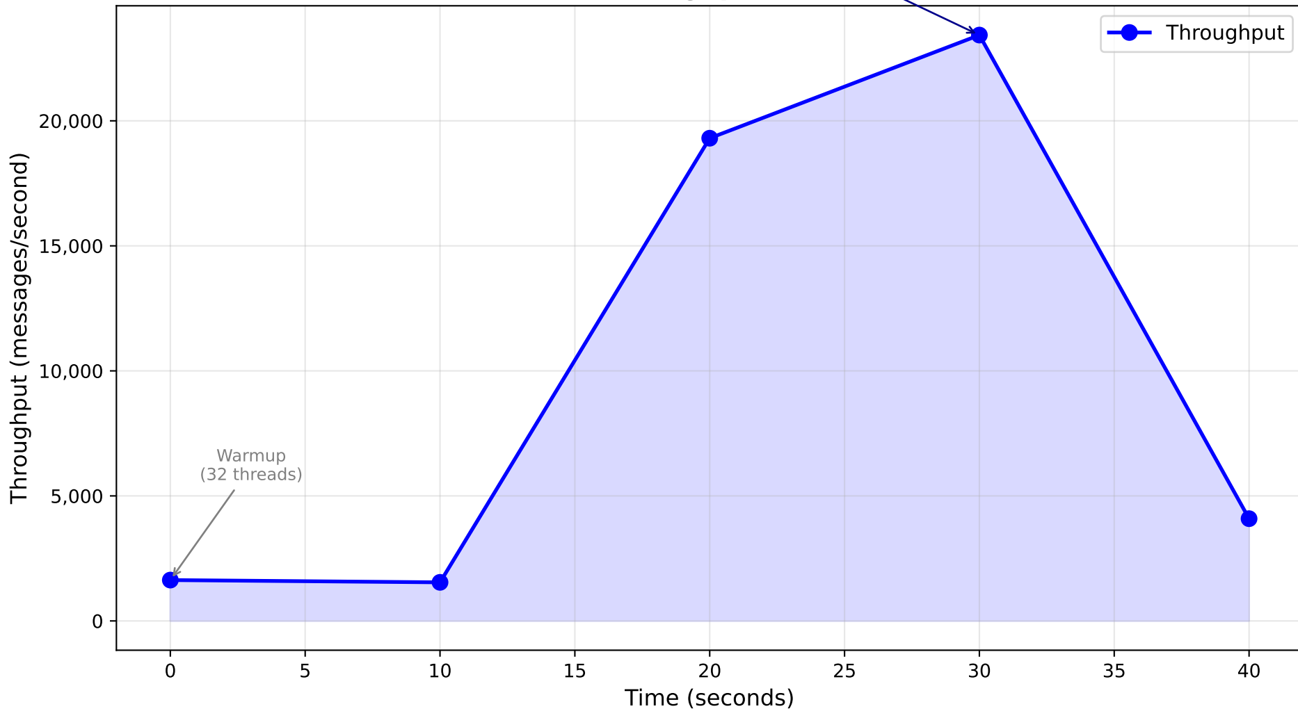
ChatFlow Load Test - Throughput Over Time (10s buckets)
