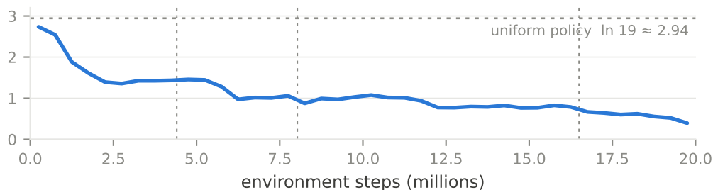
Policy entropy (nats)
