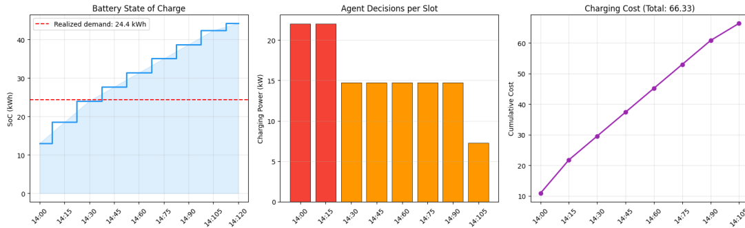
Figure 15: Example evaluation episode: SoC, charging power, and cost per 15-minute slot from 2 p.m. to 4 p.m.
