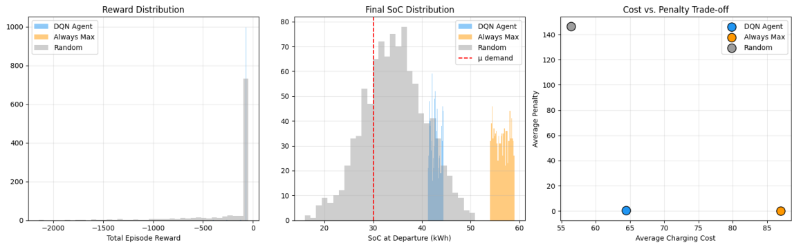
Figure 4: Distributions over 1,000 evaluation episodes: total reward, final SoC, and cost vs. penalty, compared across DQN Agent, Always-Max, and Random.
