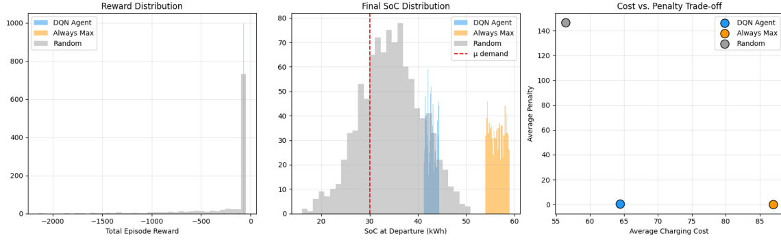
Figure 14: Distributions over 1,000 evaluation episodes: total reward, final SoC, and cost vs. penalty, compared across DQN Agent, Always-Max, and Random.
