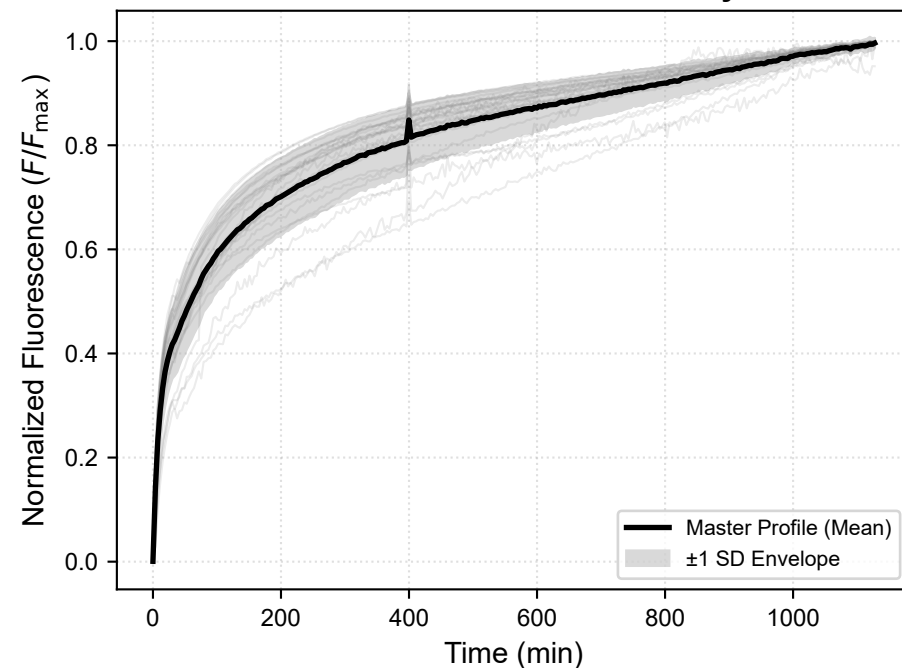
D. Normalized Kinetic Invariance Overlay
