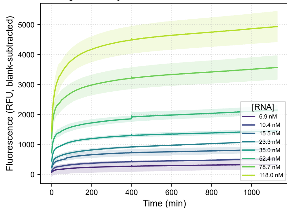
A. Target RNA Hybridization Kinetics
