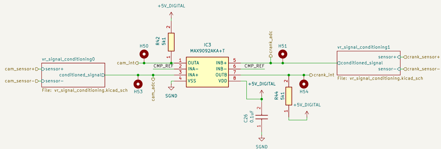
Comparator circuit
