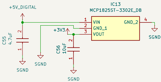
LDO for SD card
