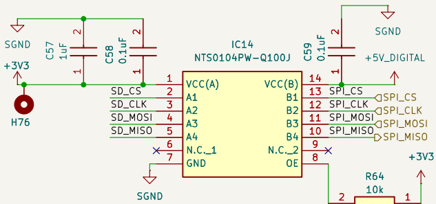
Level Shifter 5V-->3.3V
