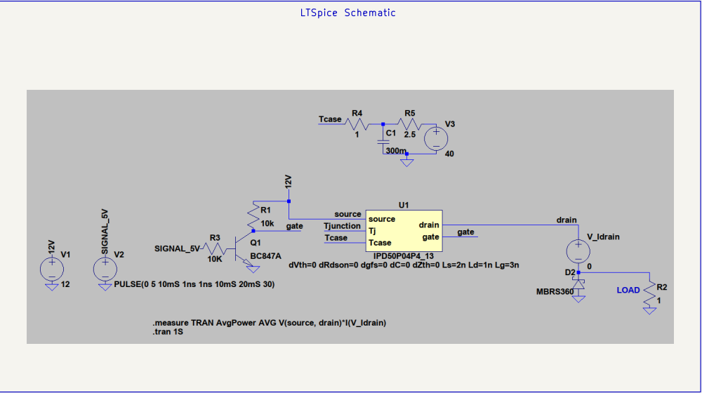
LTSpice Schematic
