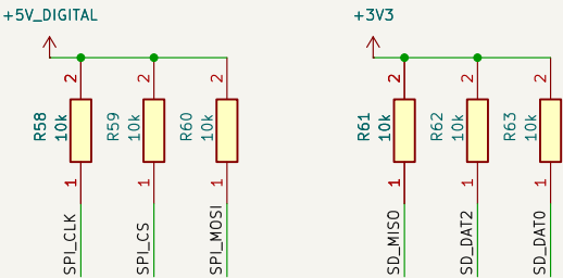
Data lines pull-ups
