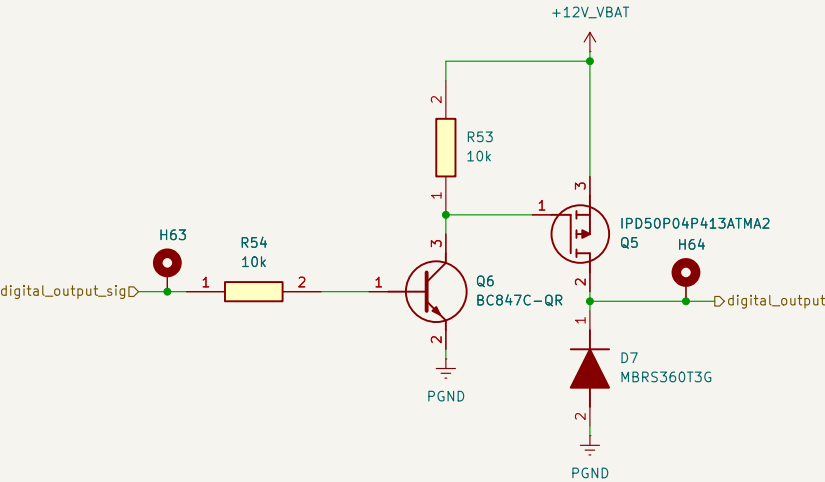
KiCad Schematic
