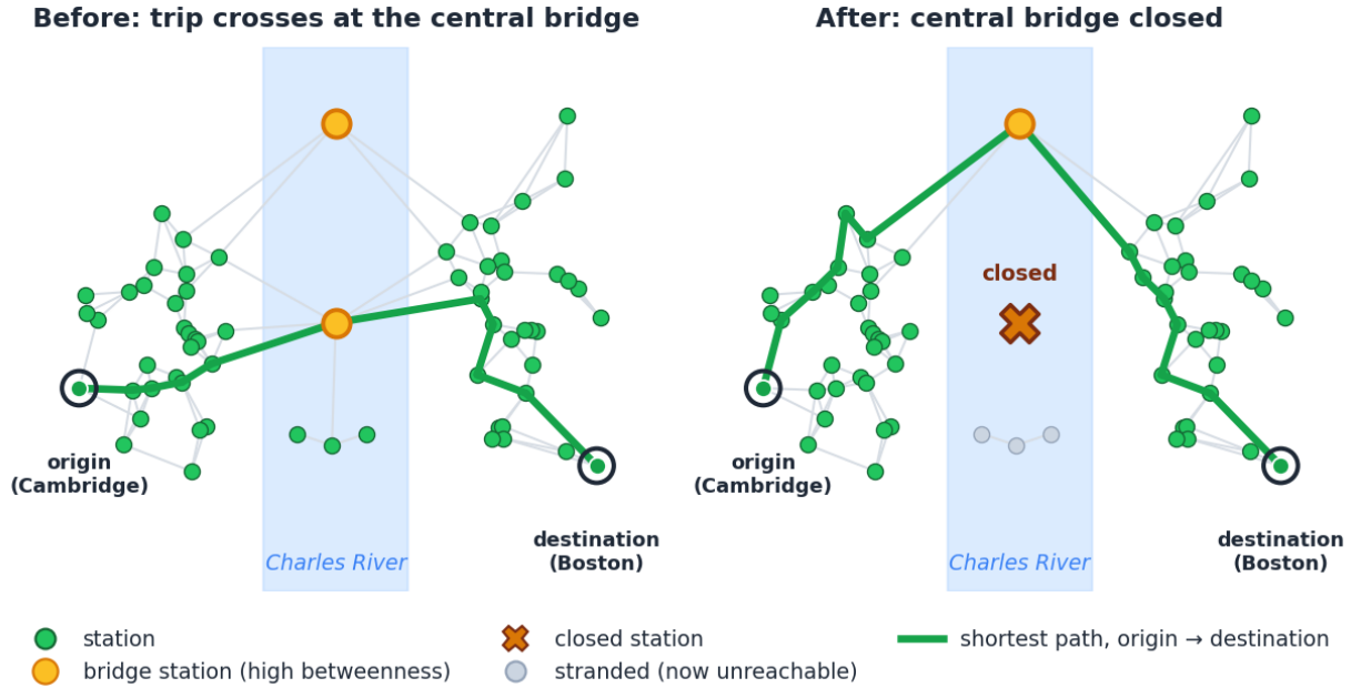
Figure 2: Figure 2. Why a low-traffic bridge station is load-bearing. Left: the shortest Cambridge-to-Boston path crosses at the central bridge station (high betweenness, modest traffic). Right: close that one station and the path detours all the way around the northern bridge, while a pocket of nearby stations is cut off from the network entirely. Layout is illustrative; the effect is the +65% in Figure 1.
