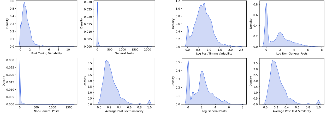
Figure 4: Log transformation to prepare data for Gaussian Mixture Model
