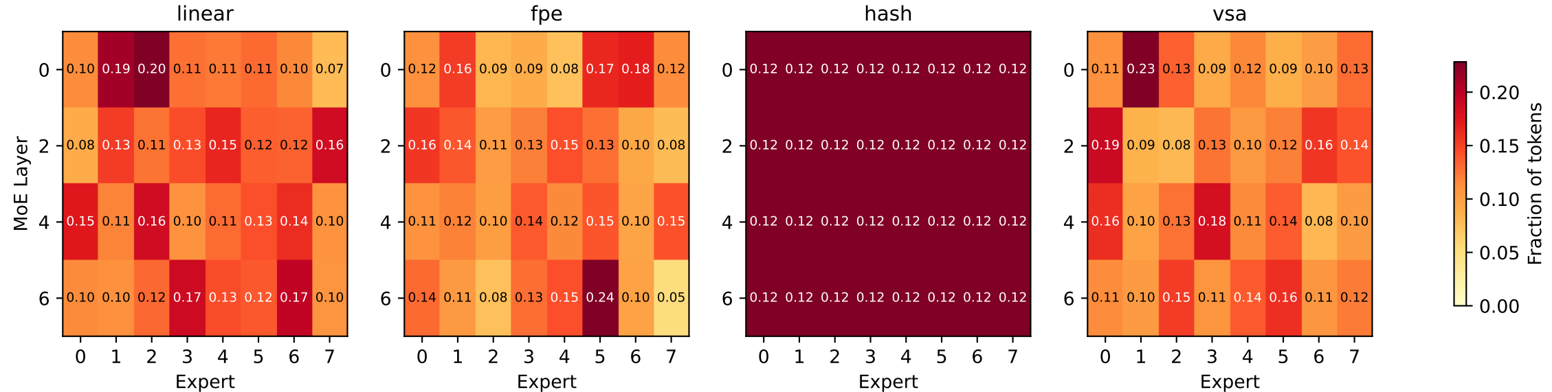
Expert Token Fraction by Layer and Router Type
