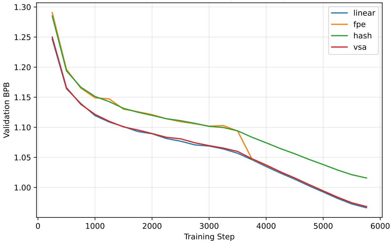
Validation Loss During Pretraining
