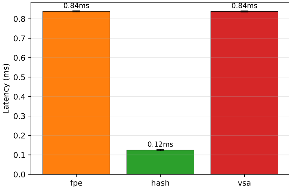
Router Latency per Forward Call (B×T=8192 tokens)
