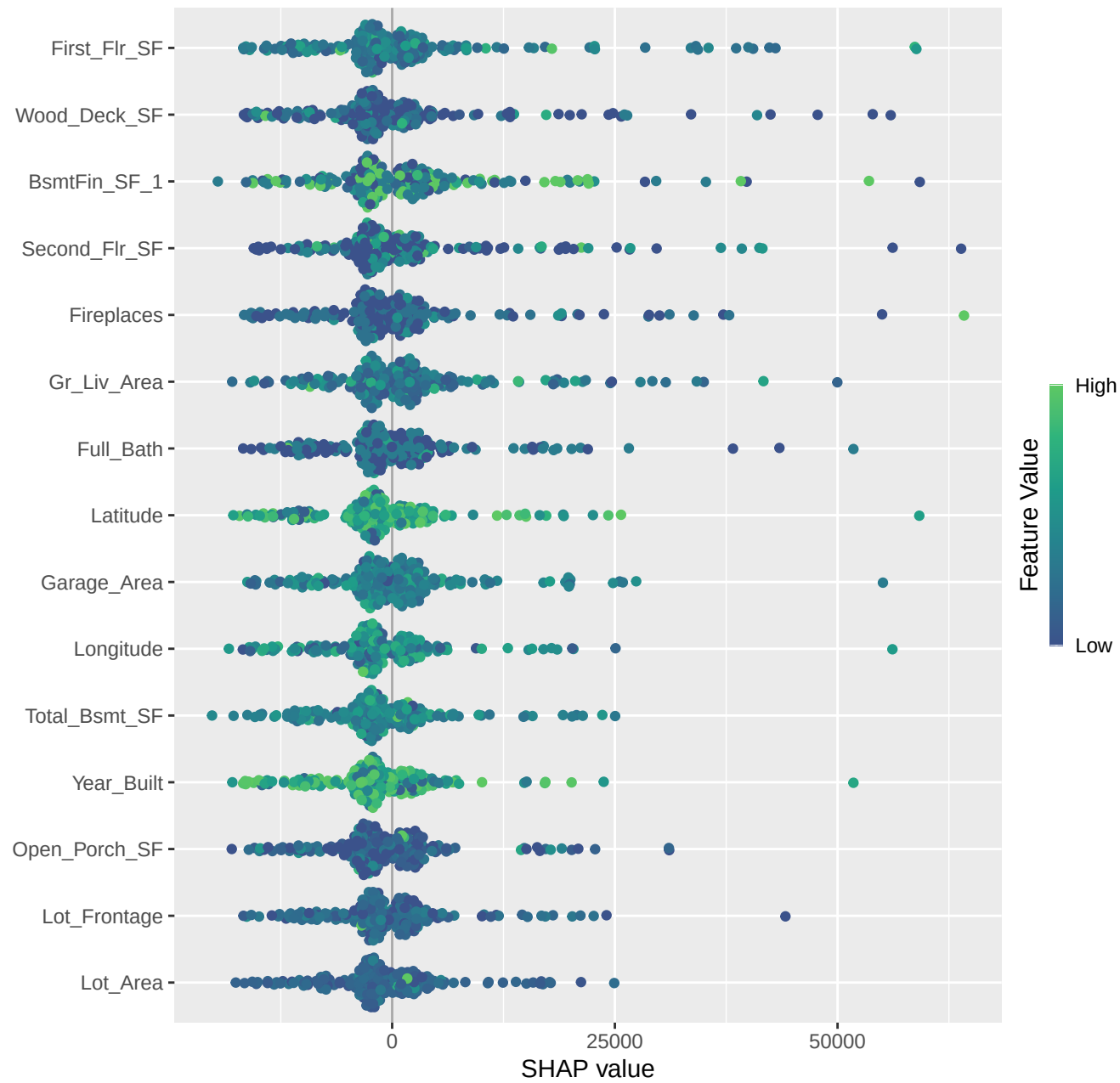
Feature Importance
