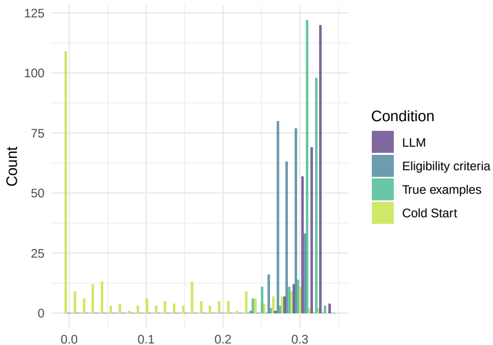
Relevant records found by condition – van_de_Schoot_2018
