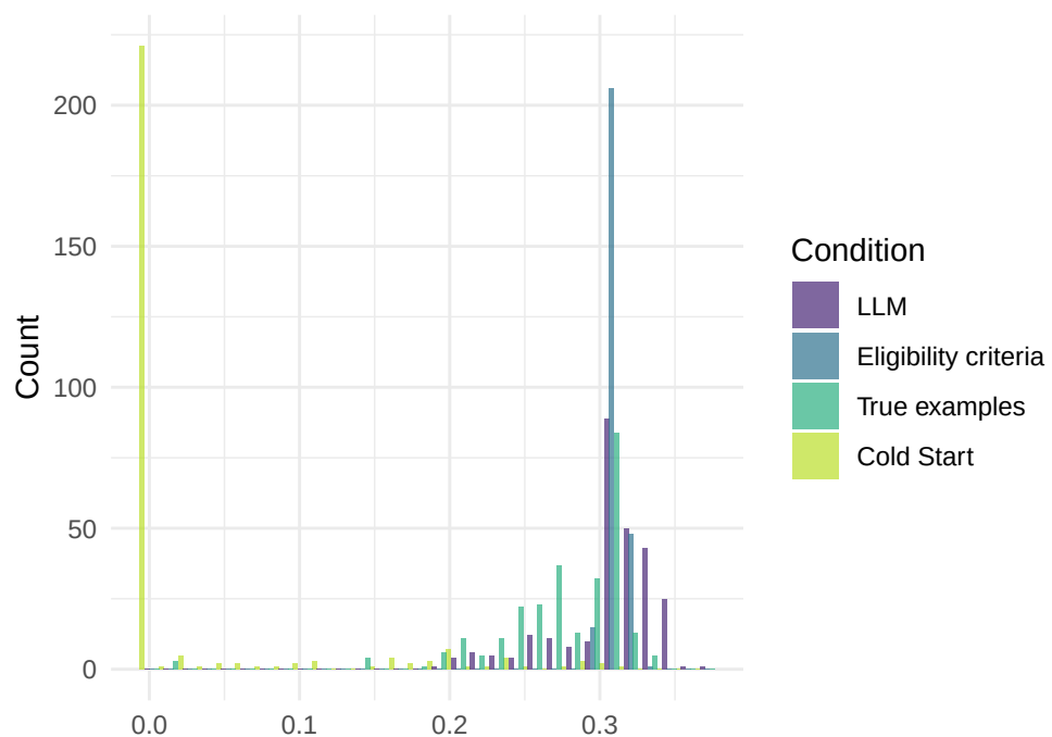
relevant records found by condition – Brouwer_2019
