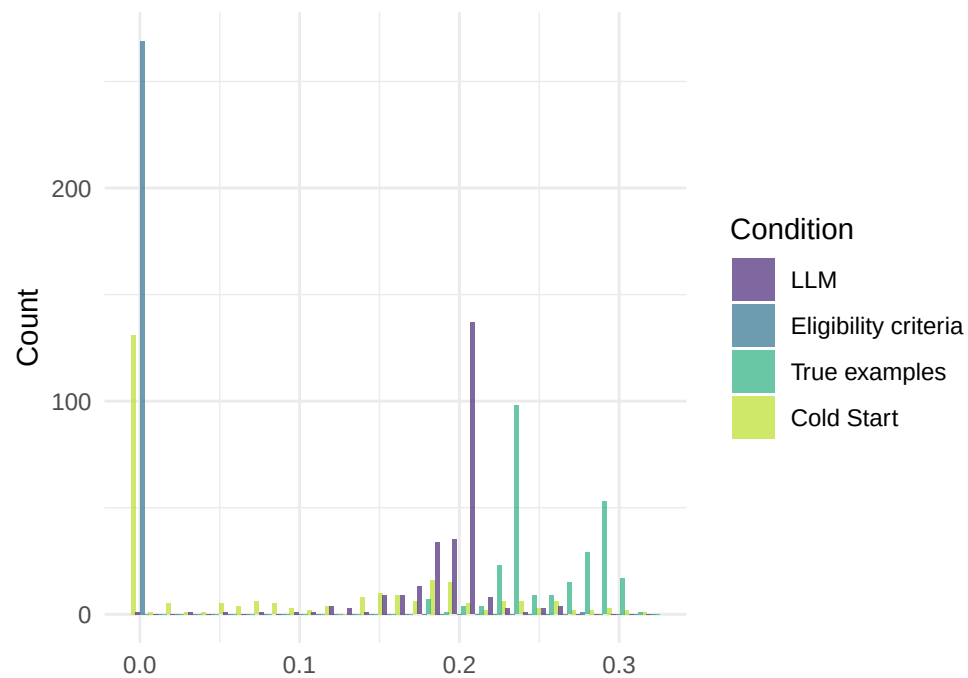
N relevant records found by condition – Radjenovic_2013
