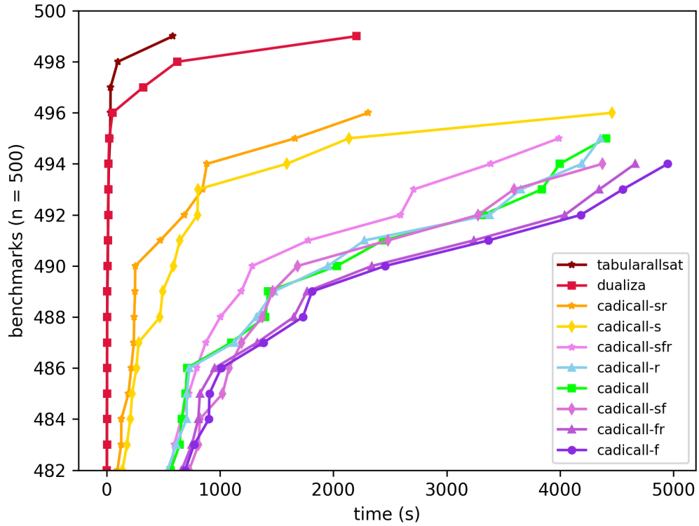
Figure 4: TabularAllSat vs. CaDiCall Close Up
