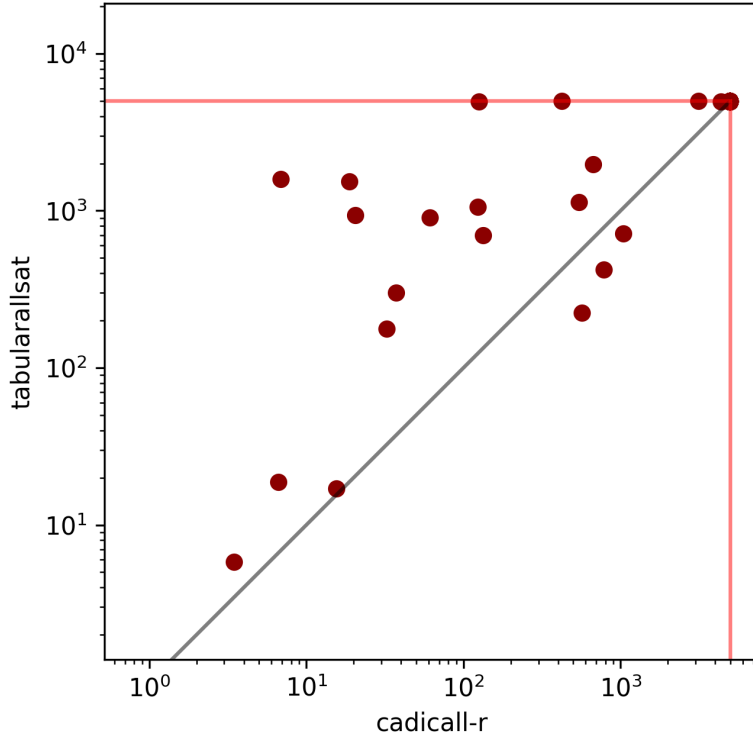
Figure 11: TabularAllSat vs CaDiCaL r
