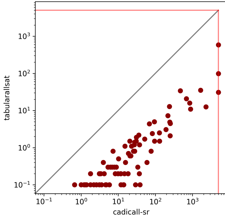
Figure 5: TabularAllSat vs. CaDiCaL
