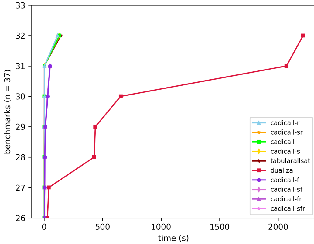
Figure 2: Custom Benchmarks.
