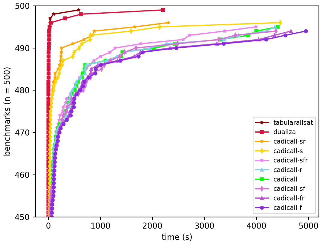
Figure 1: TabularAllSat Benchmarks.
