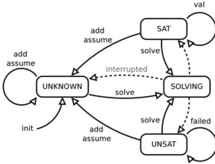
Figure 1: The four possible states of SAT solvers according to the IPASIR interface (see [? ]).
