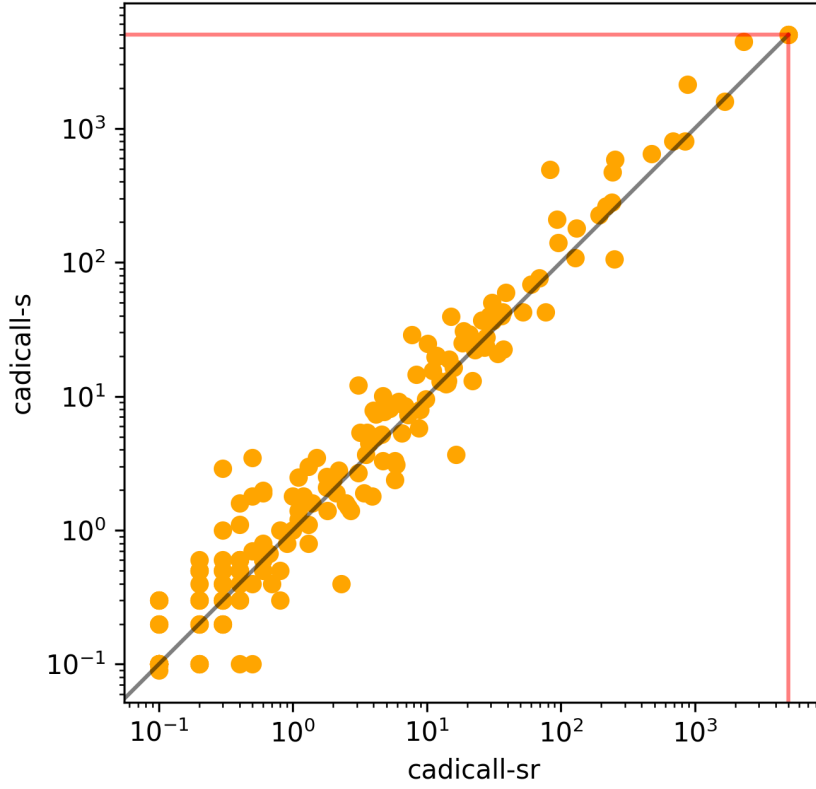
Figure 6: CaDiCaL sr vs s
