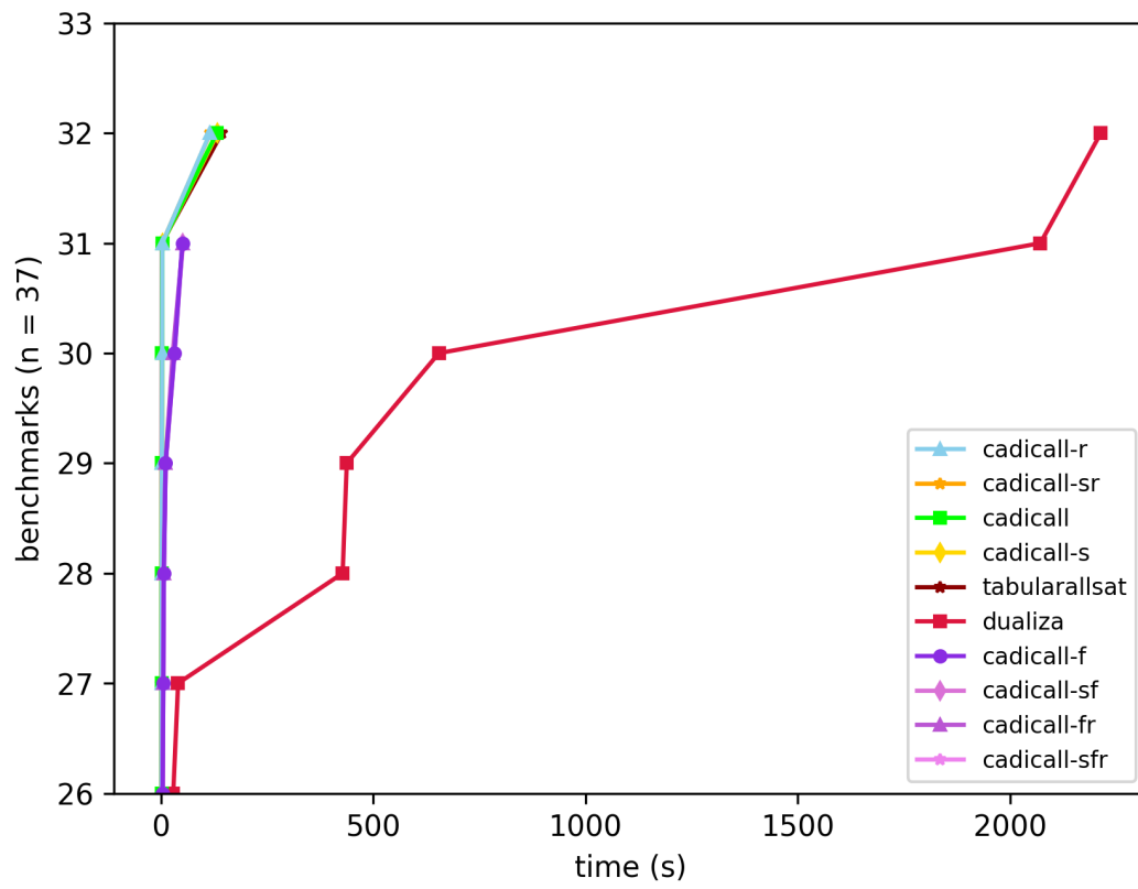
Figure 2: All Custom Benchmarks
