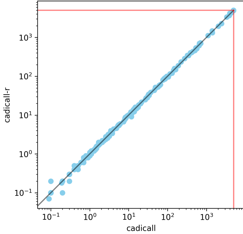
Figure 7: CaDiCaL vs CaDiCaL r
