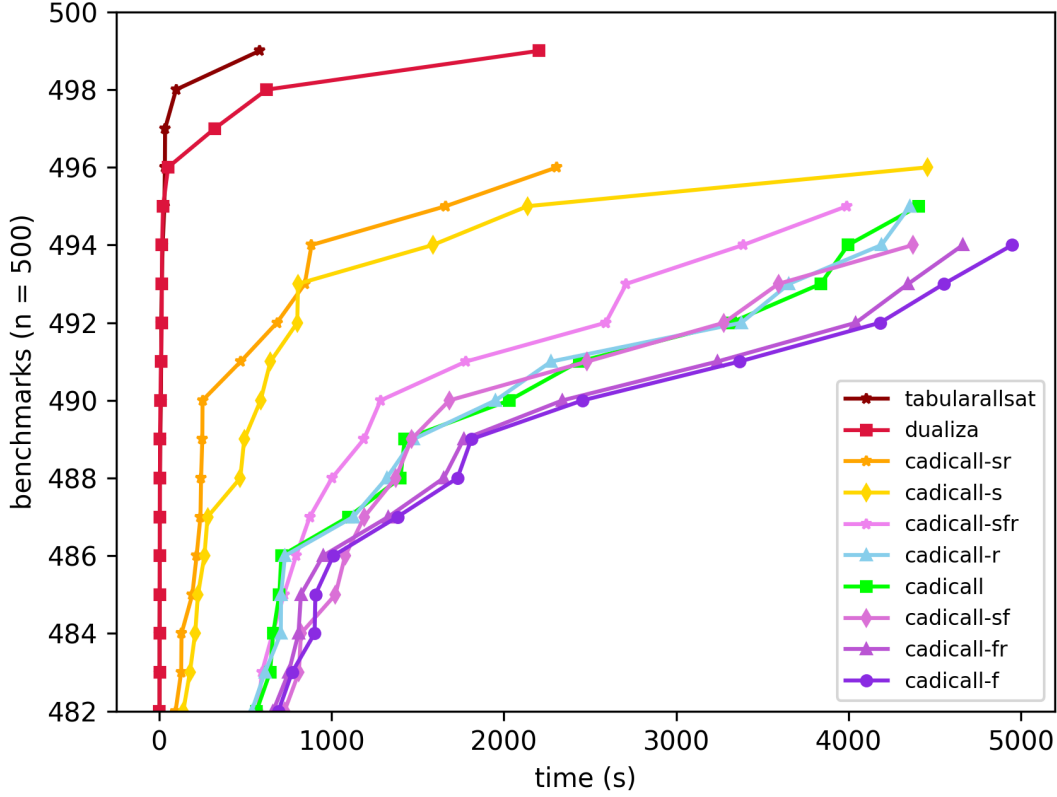
Figure 4: TabularAllSat vs. CaDiCaL Close Up
