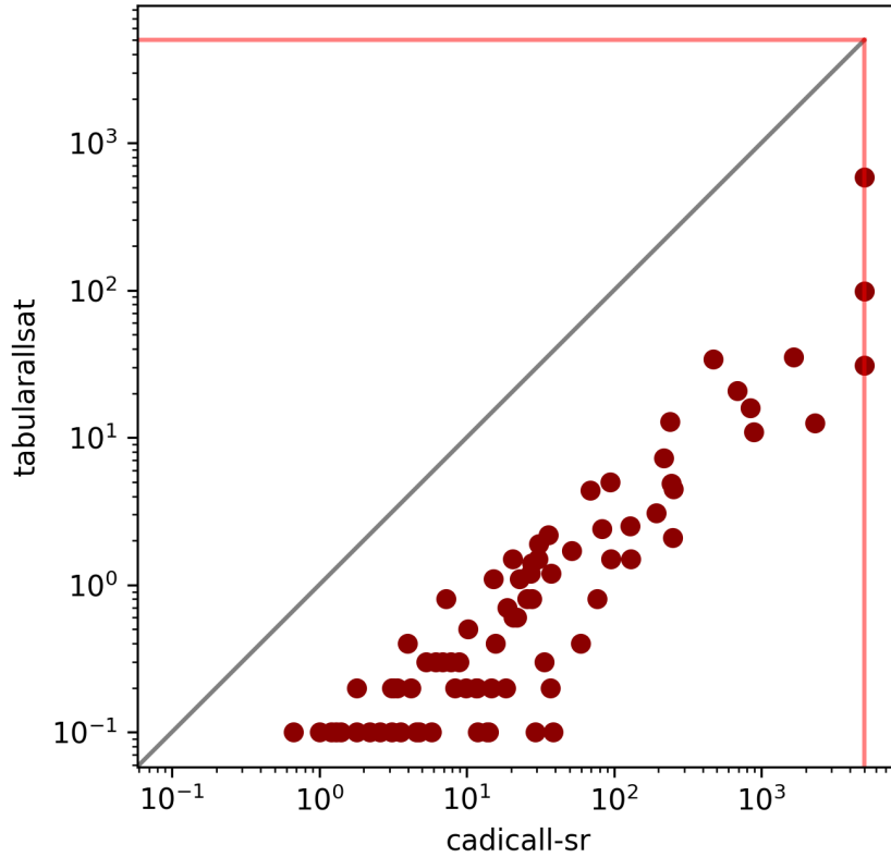
Figure 5: TabularAllSat vs. CaDiCaL
