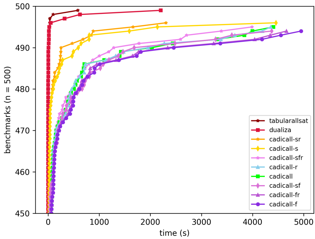
Figure 1: Benchmarks from TabularAllSat
