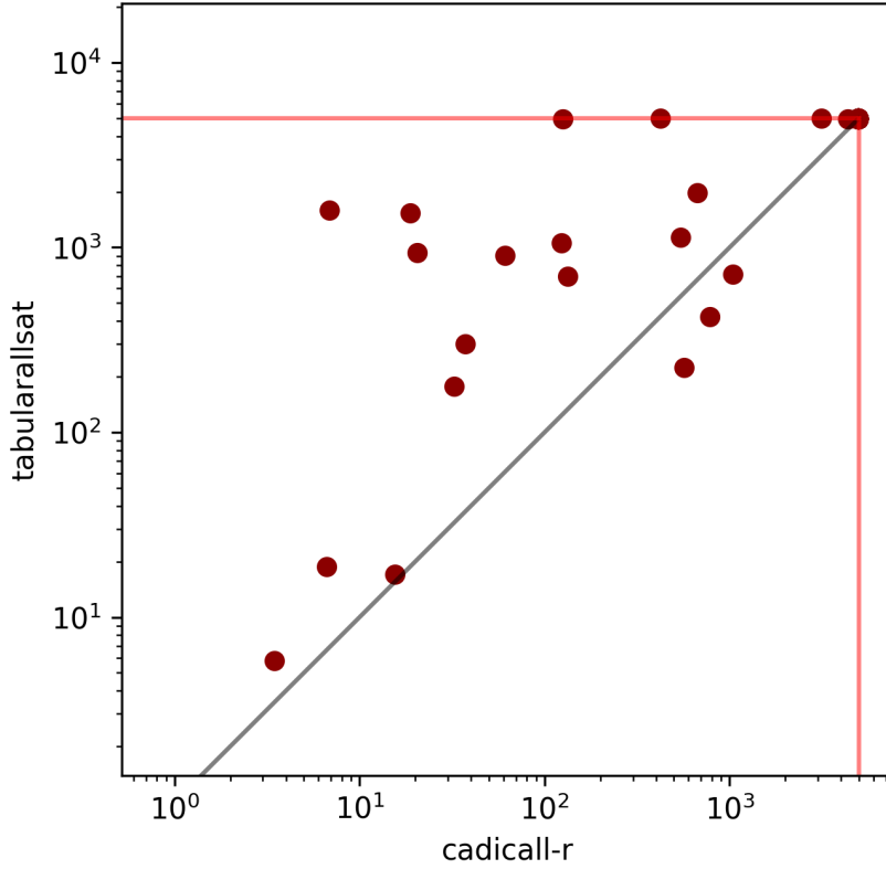
Figure 11: TabularAllSat vs CaDiCaL r
