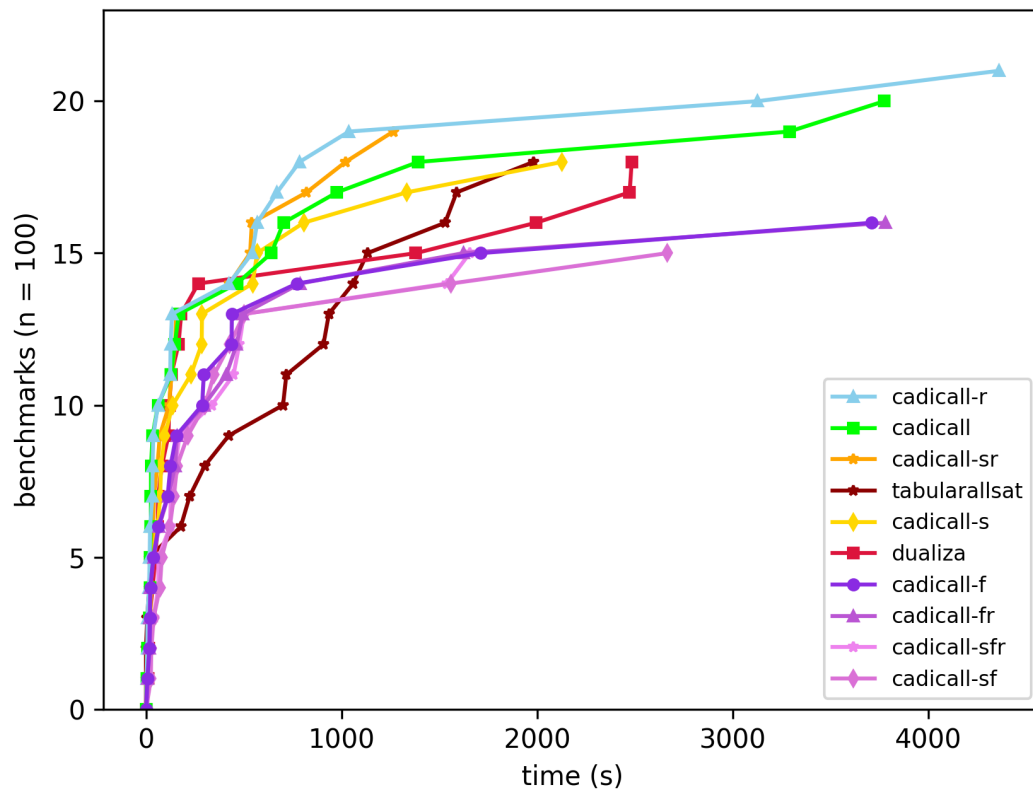
Figure 3: All Model Count Competition benchmarks
