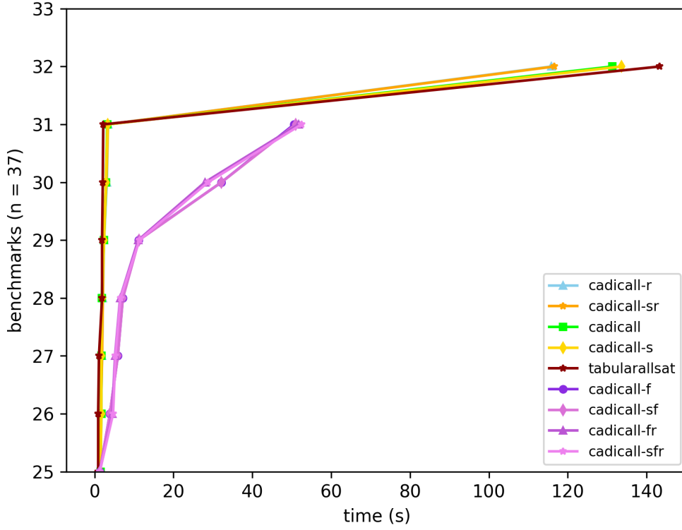
Figure 8: All Custom Benchmarks Close Up
