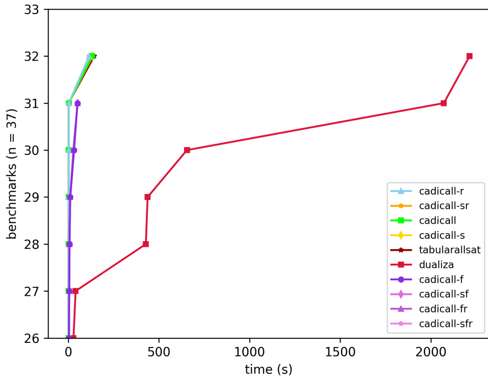
Figure 2: All Custom Benchmarks
