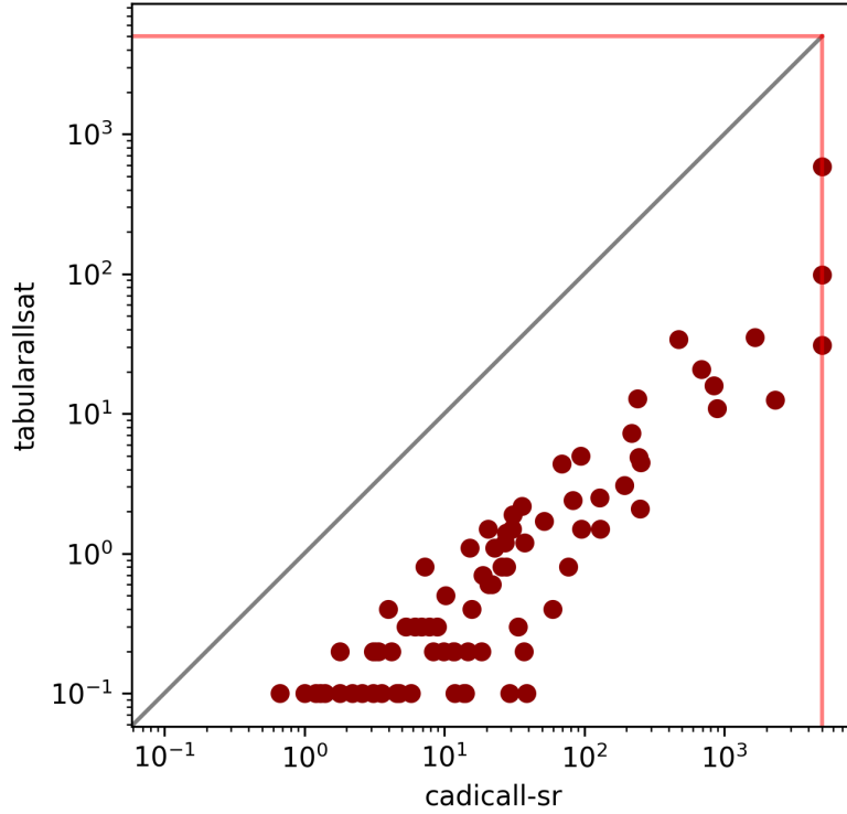
Figure 5: TabularAllSat vs. CaDiCAll
