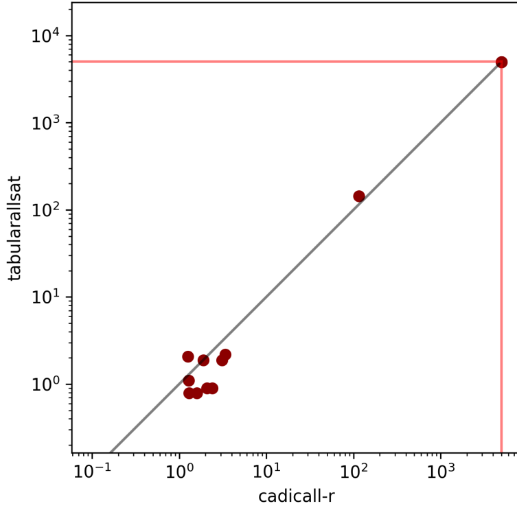
Figure 9: TabularAllSat vs CaDiCall r
