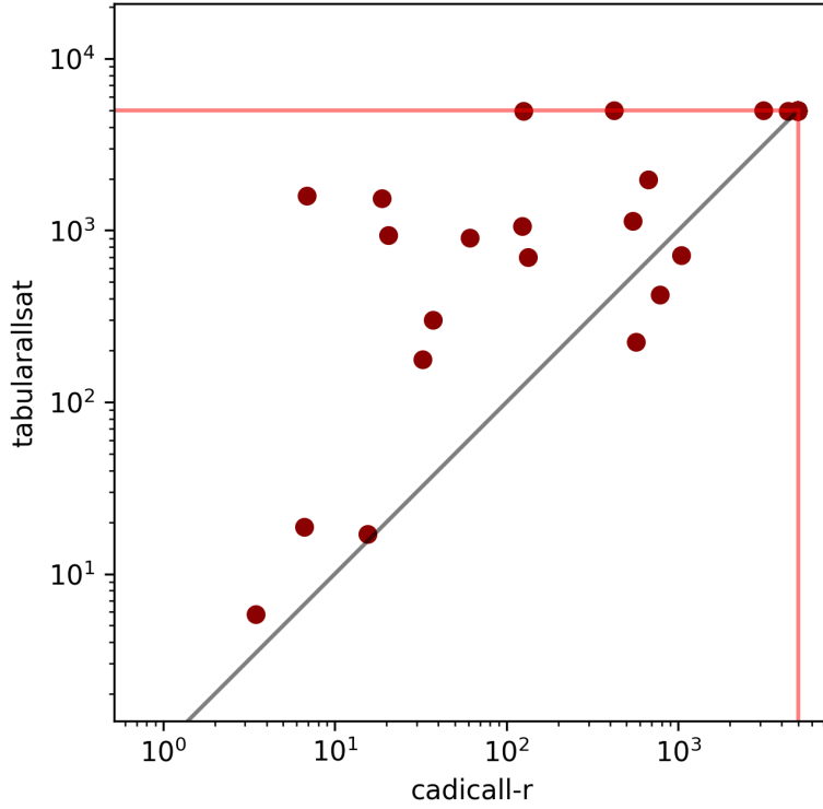
Figure 11: TabularAllSat vs CaDiCaL r
