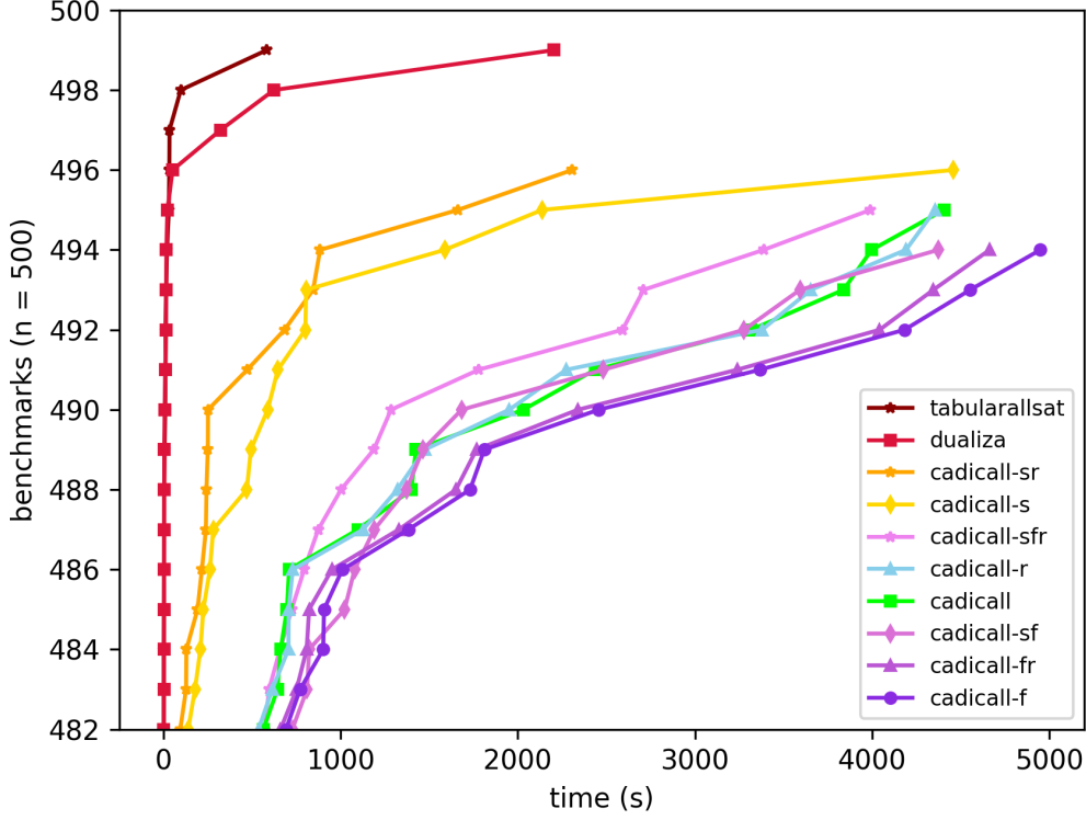
Figure 4: TabularAllSat vs. CaDiCaL Close Up
