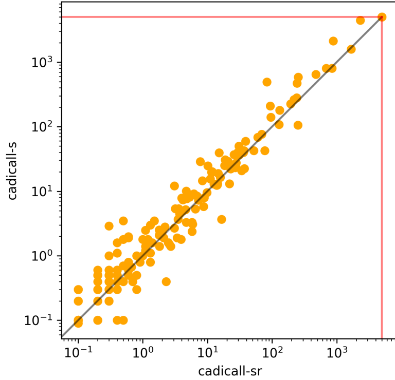
Figure 6: CaDiCaL sr vs s
