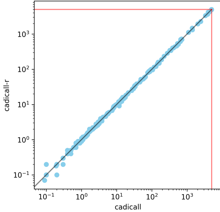
Figure 7: CaDiCaL vs CaDiCaL r
