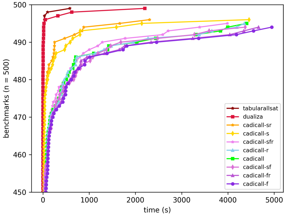
Figure 1: Benchmarks from TabularAllSat
