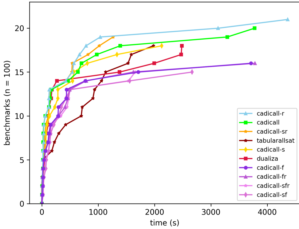
Figure 3: All Model Count Competition Benchmarks
