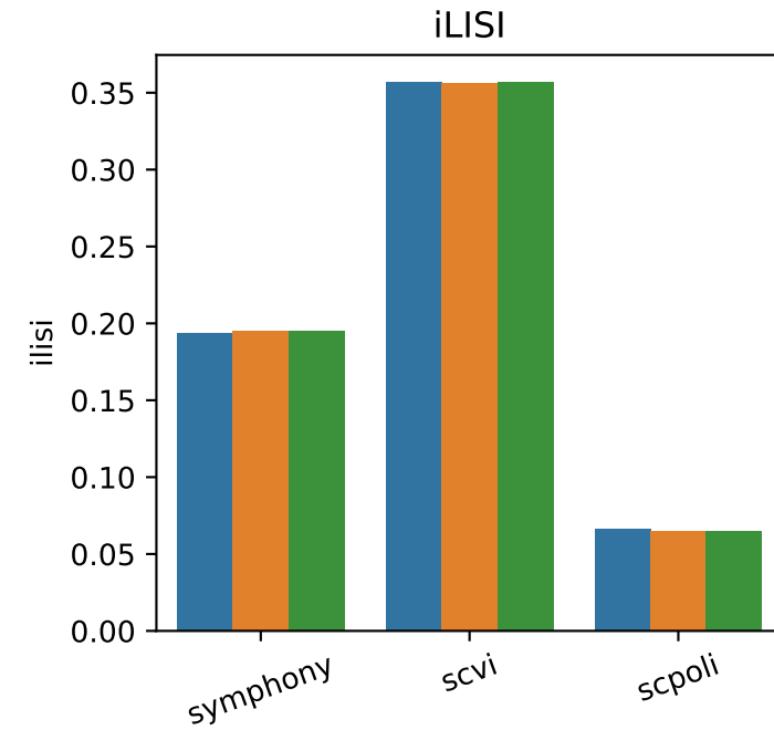
Reference mapping metrics — Exp2 (wave2 source_5)
