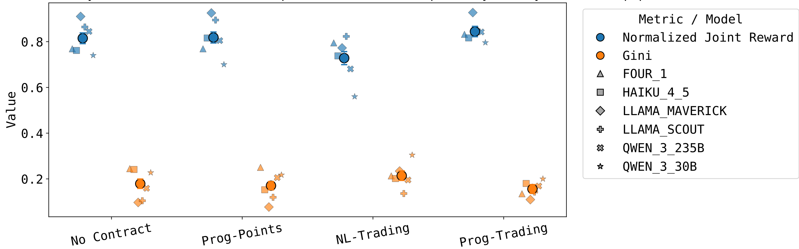
Joint reward and Gini by contract (buckets=['Independent', 'Mutual Dependency', 'Asymmetric'], p4p=False)
