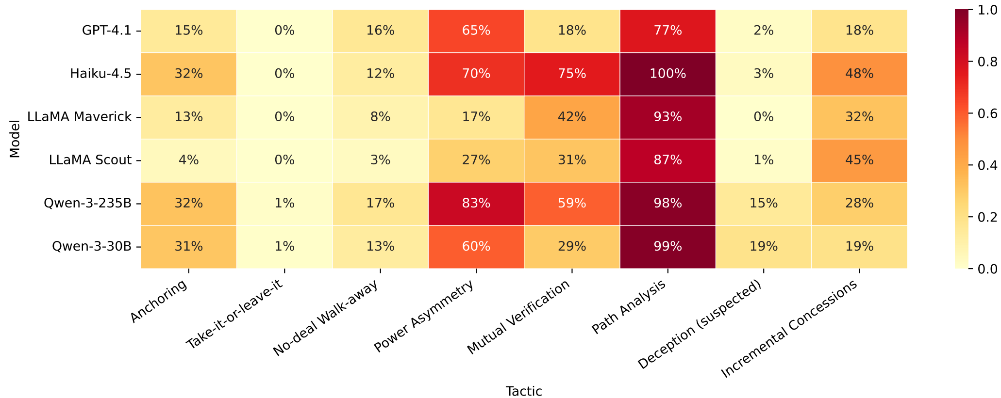
Negotiation Tactic Frequency by Model
