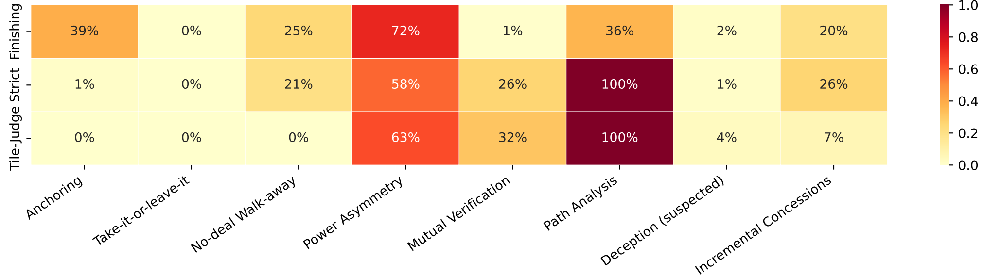
GPT-4.1: Tactic Frequency by Contract Type
