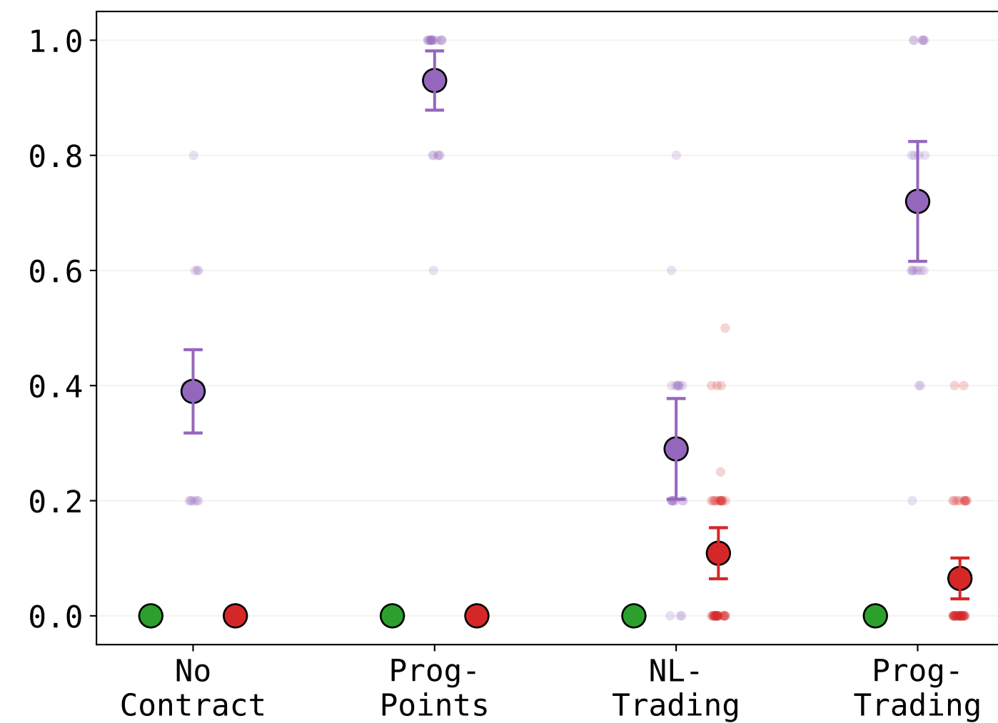
Both Beat Baseline
