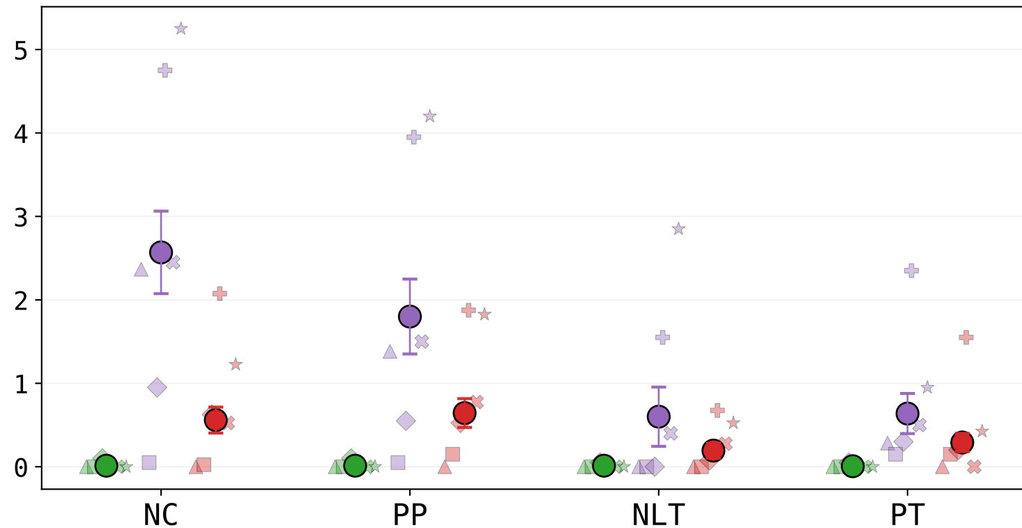
Defection Volume
