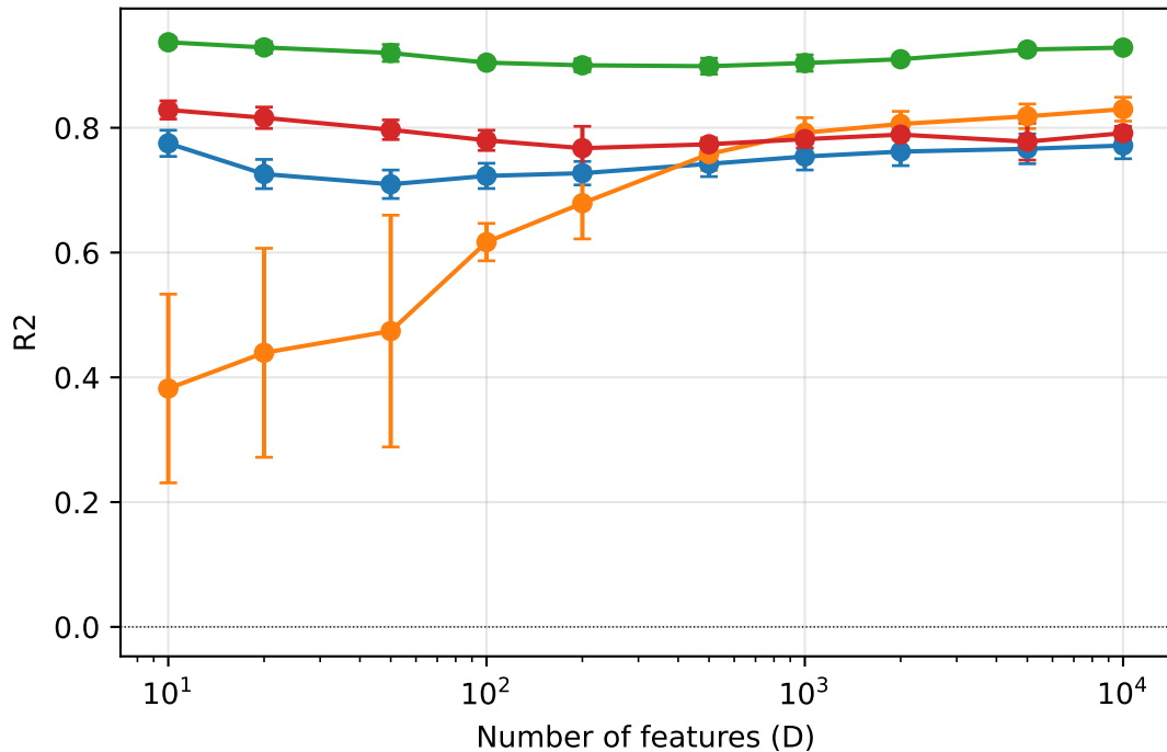
5 causal features regardless of D (ambient dimensionality only)
