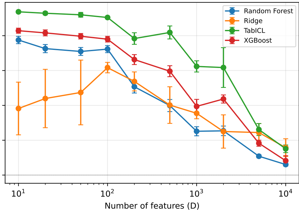
Causal features scale with D (5% of D) (signal dimensionality grows too)
