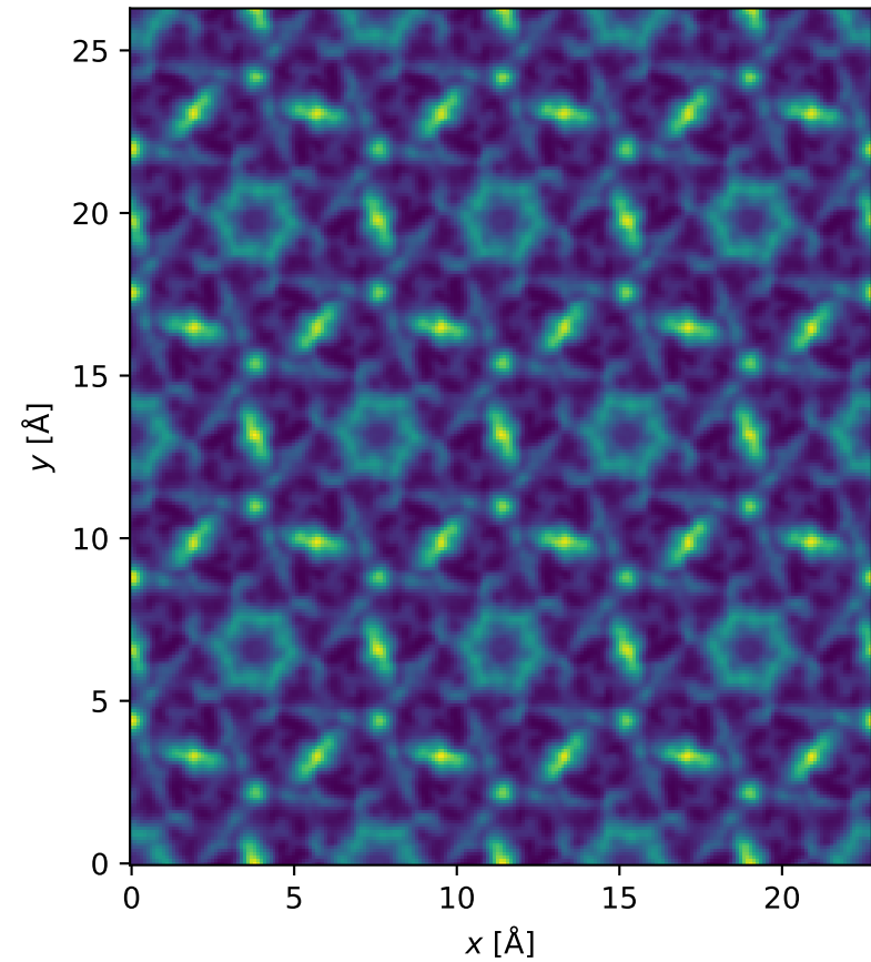
Uncorrected TEM image
