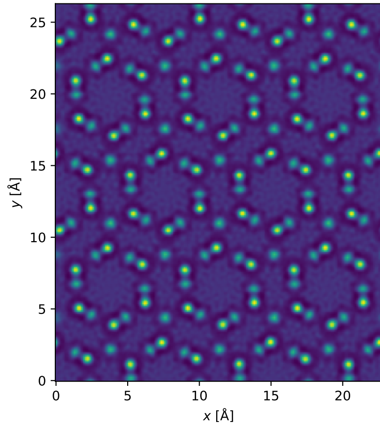
Aberration-Corrected TEM image
