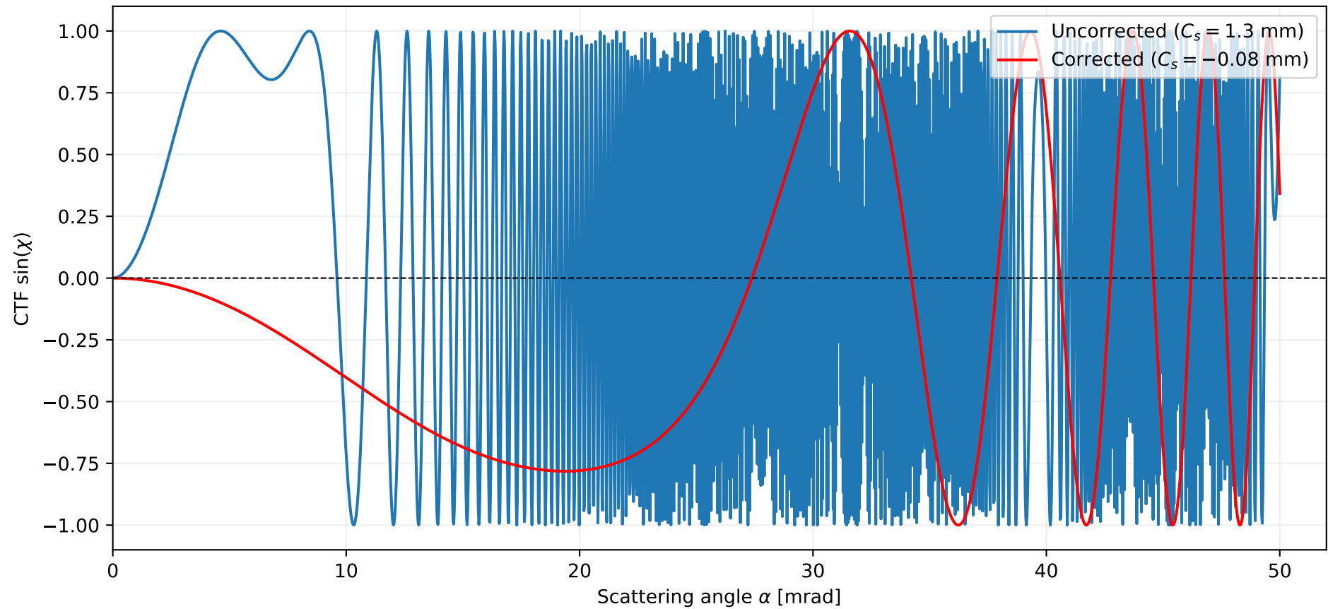
CTF: Inner Function Evaluation ( \sin \chi )
