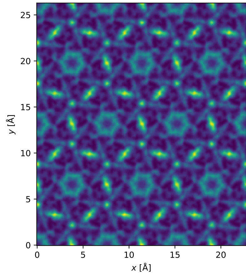
Uncorrected TEM image
