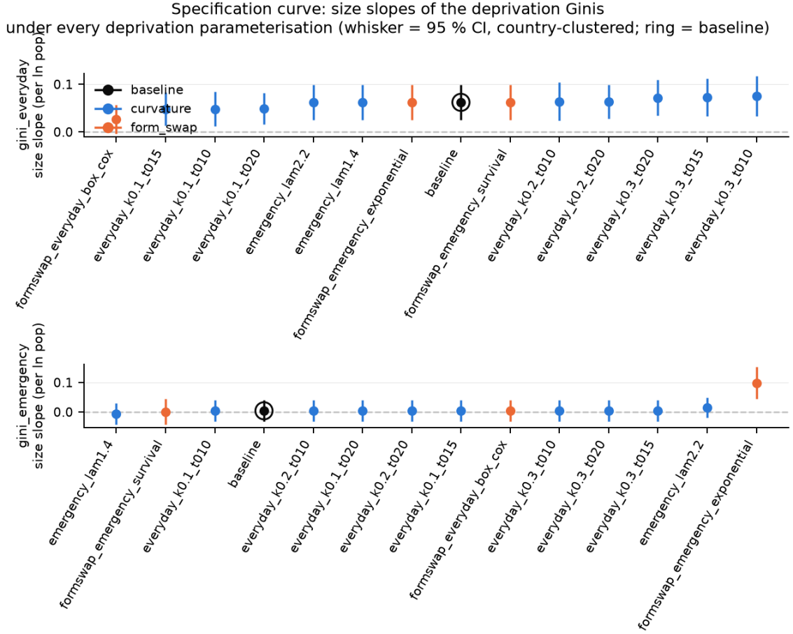
Figure S2: Specification curve of the inequality-scaling slopes. Top: everyday Gini; bottom: emergency Gini. Each point is the size elasticity of the within-city Gini re-estimated under the ringed baseline or one of the 14 alternative deprivation parameterisations (blue: curvature grid; orange: functional-form swaps); whiskers are country-clustered 95 % CIs. The everyday-Gini slope is positive under every specification (+0.026 to +0.075; significant in 13/14, the exception being the concave Box-Cox form swap at p = 0.083 ). The emergency-Gini slope splits by beyond-cut-off escalation form: flat under saturating and polynomial escalation, rising only under exponential escalation (+0.098, p = 0.0003 ).
