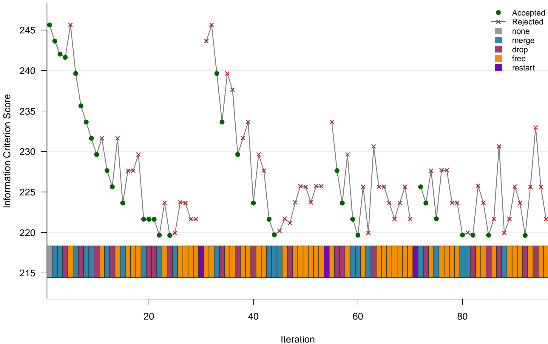
Simulated Annealing Trace
