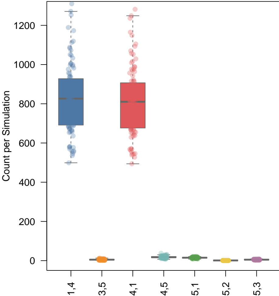
Distribution of Transition Counts
