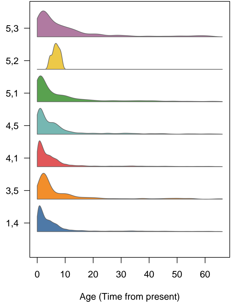
Distribution of Transition Ages
