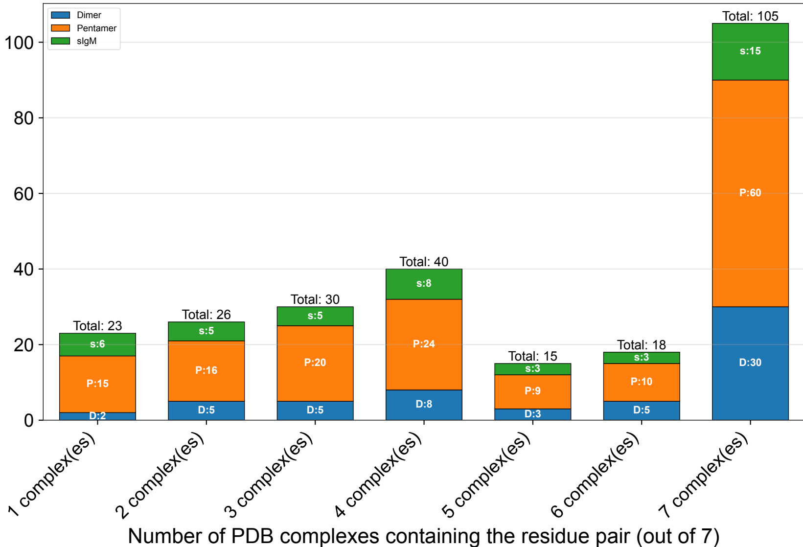
Number of residue pairs
