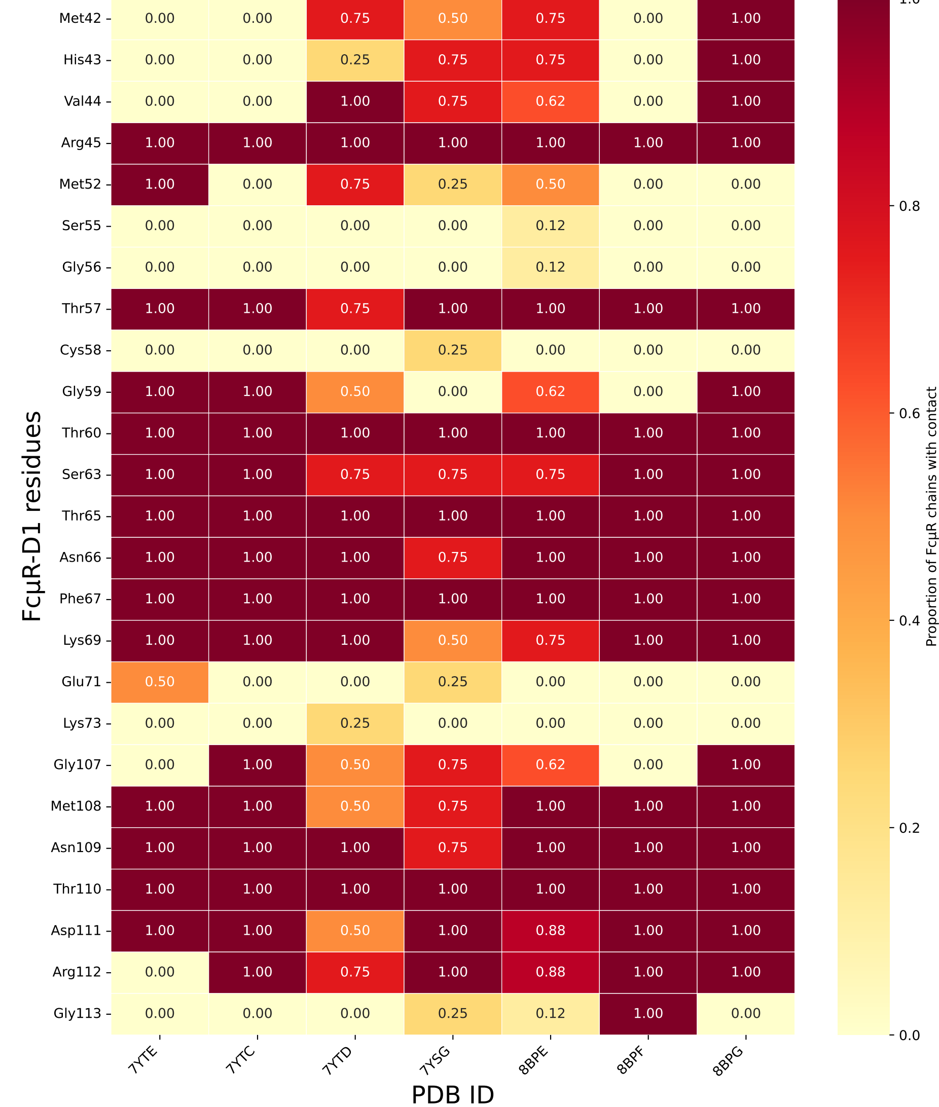
FcμR-D1 residue contact frequency across different IgM complexes
