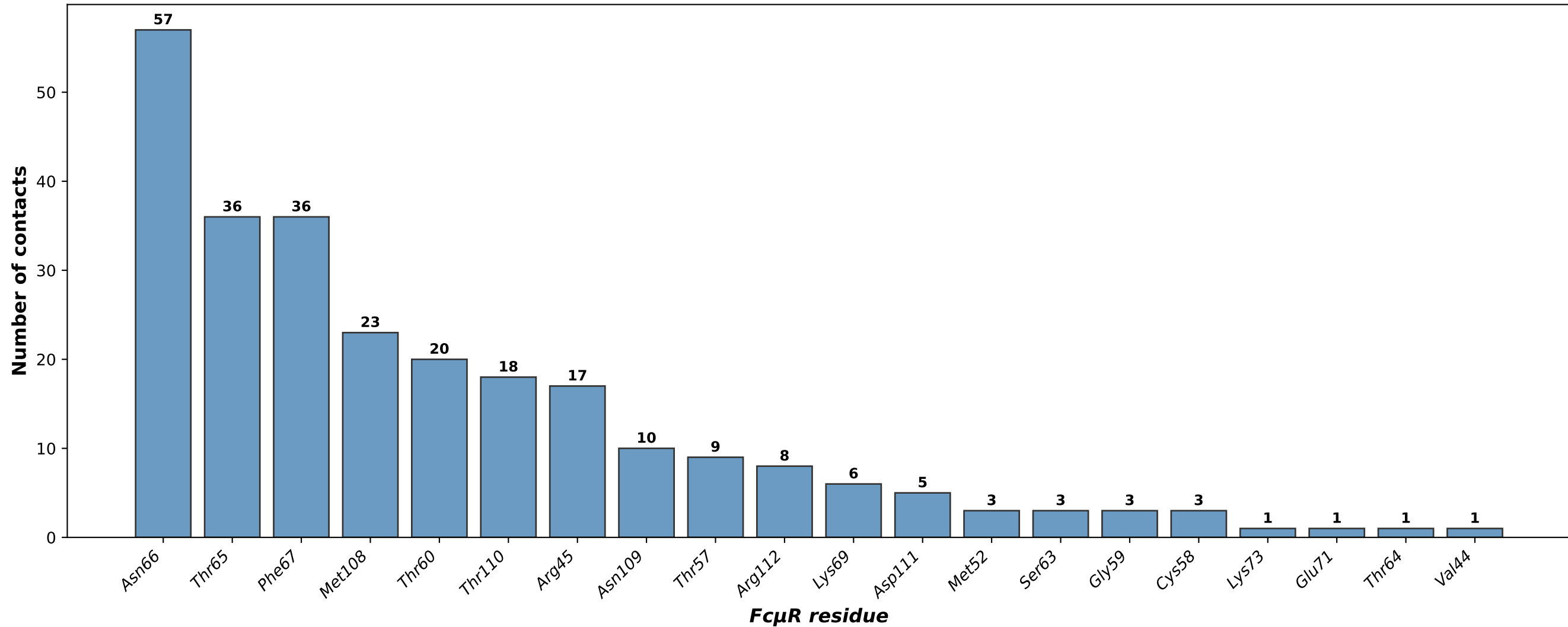
FcμR contact frequency (7 structures merged)
