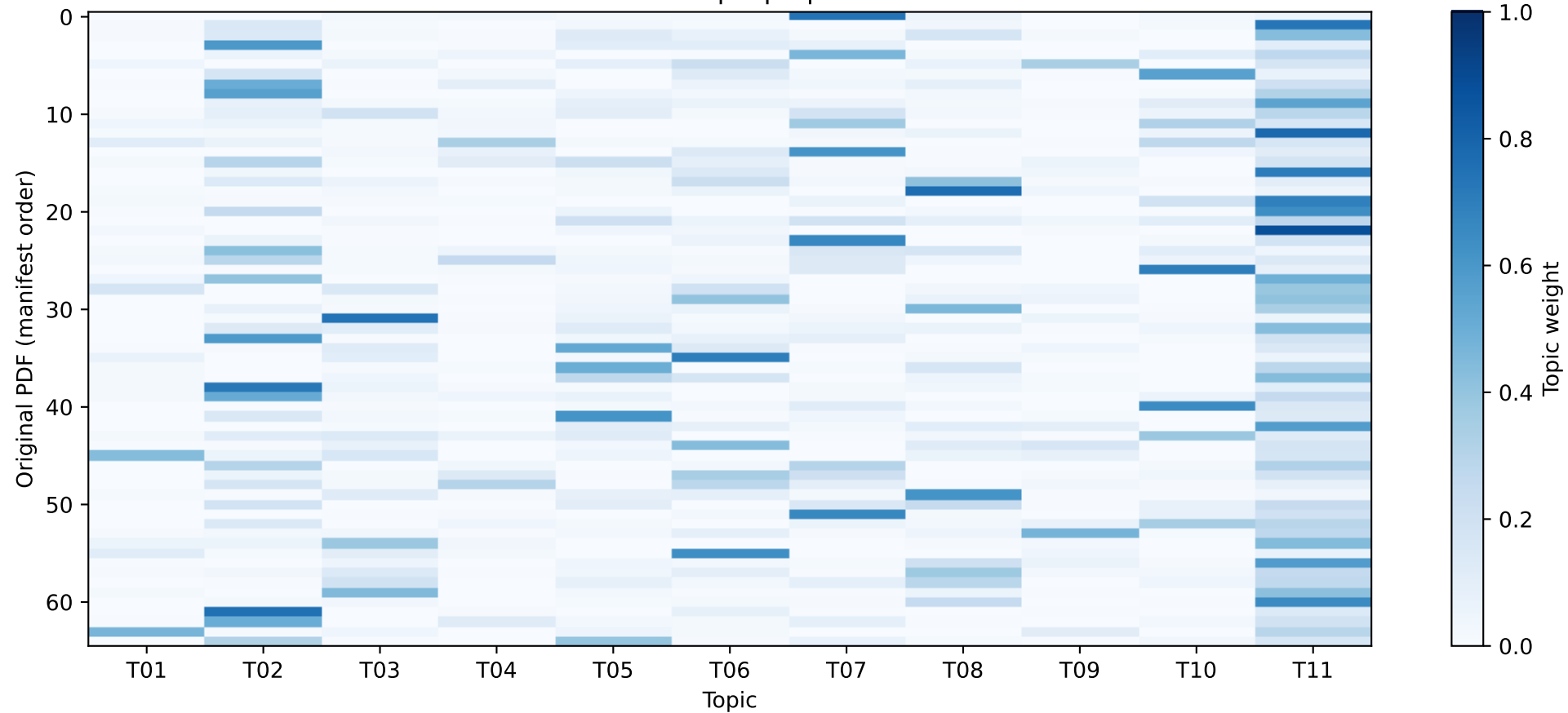
Document-topic proportions
