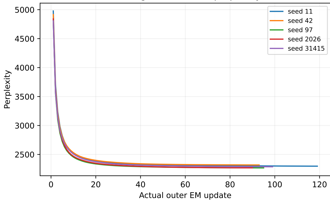
Training bound-based perplexity
