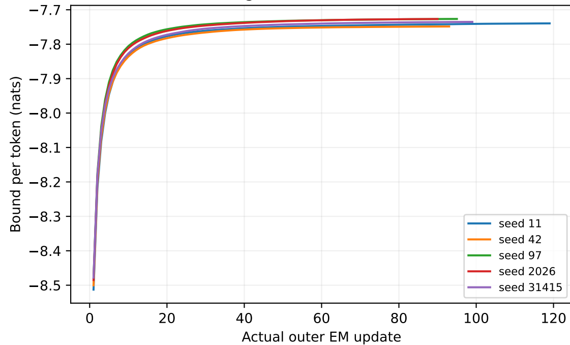
Training variational lower bound
